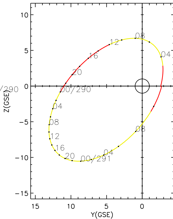
CLUSTER 2 orbit 2004 289 (10/15) 02:05 UT to 2004 291 (10/17) 11:10 UT
