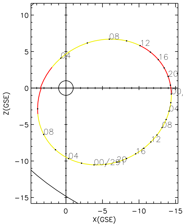
CLUSTER 2 orbit 2004 289 (10/15) 02:05 UT to 2004 291 (10/17) 11:10 UT
