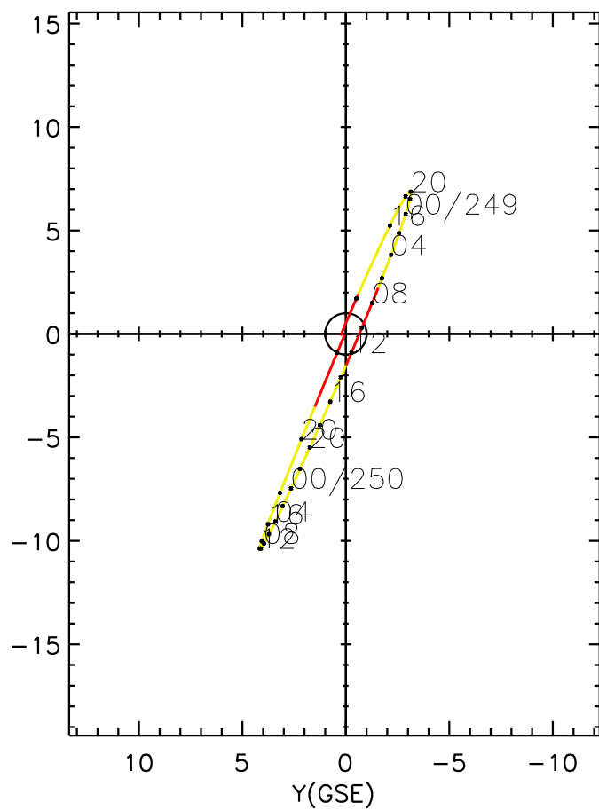
CLUSTER 2 orbit 2004 248 (09/04) 13:16 UT to 2004 250 (09/06) 22:21 UT
