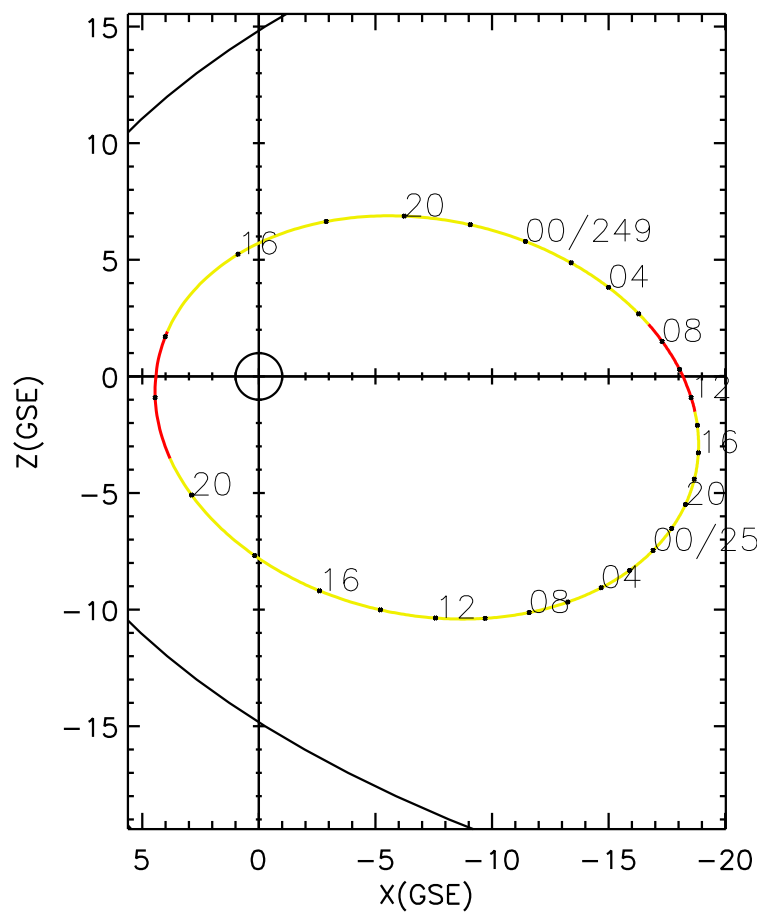
CLUSTER 2 orbit 2004 248 (09/04) 13:16 UT to 2004 250 (09/06) 22:21 UT
