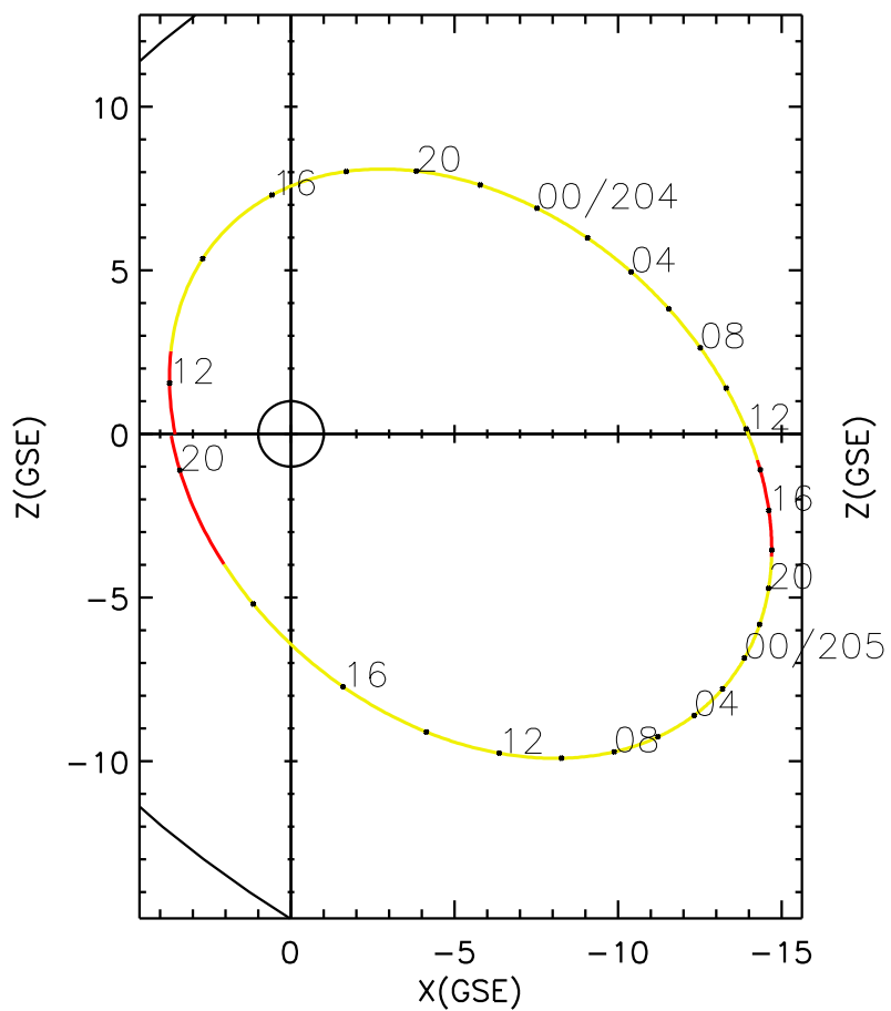
CLUSTER 2 orbit 2004 203 (07/21) 11:21 UT to 2004 205 (07/23) 20:26 UT
