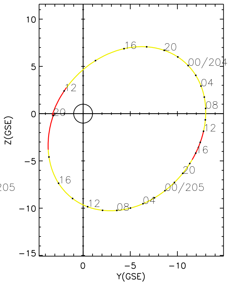
CLUSTER 2 orbit 2004 203 (07/21) 10:55 UT to 2004 205 (07/23) 20:05 UT
