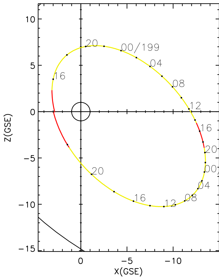
CLUSTER 2 orbit 2004 198 (07/16) 14:26 UT to 2004 200 (07/18) 23:31 UT
