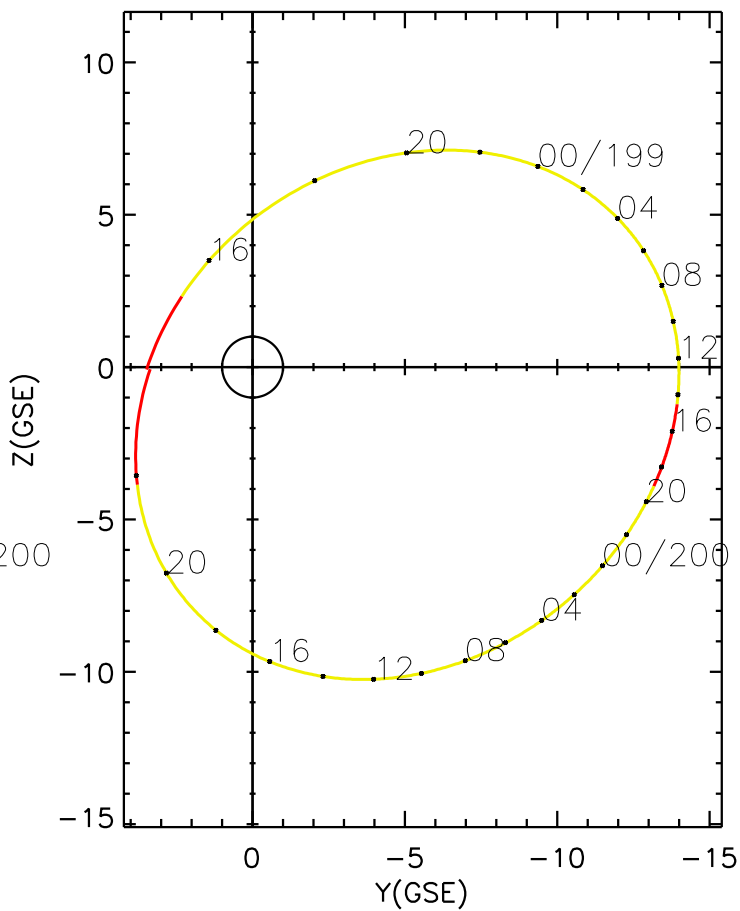
CLUSTER 2 orbit 2004 198 (07/16) 14:26 UT to 2004 200 (07/18) 23:31 UT
