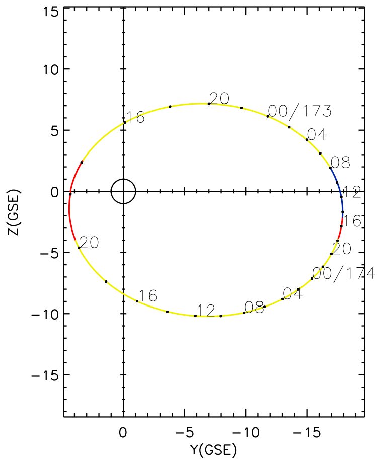
CLUSTER 2 orbit 2004 172 (06/20) 13:00 UT to 2004 174 (06/22) 22:05 UT
