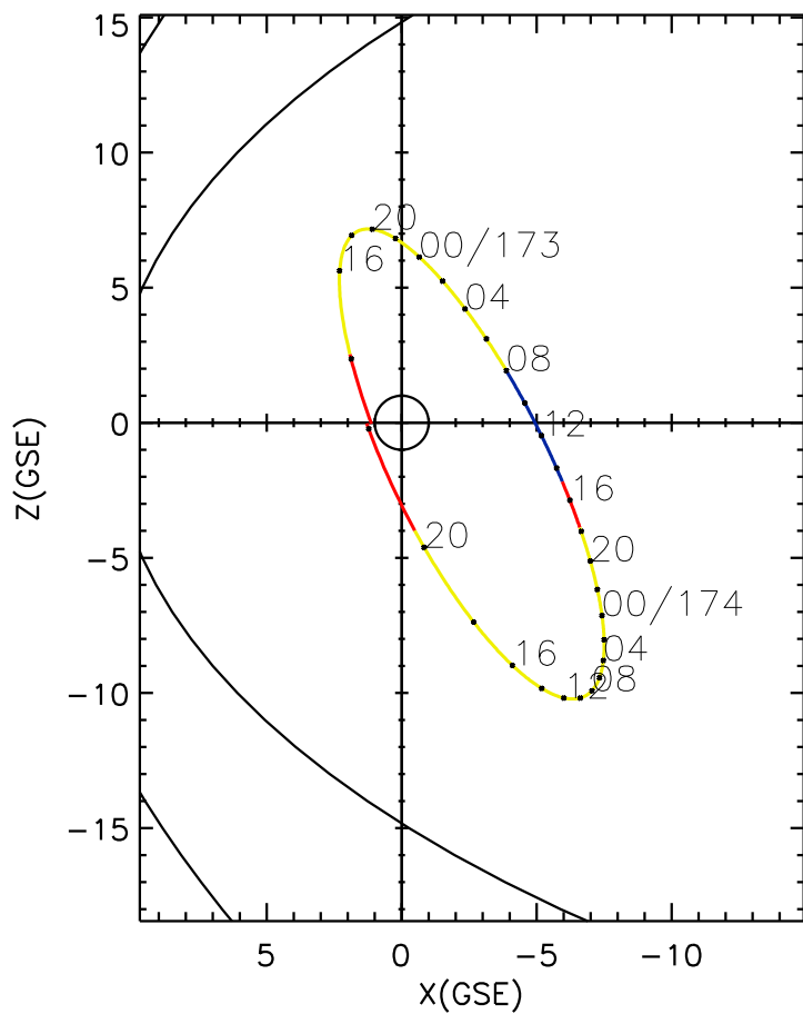
CLUSTER 2 orbit 2004 172 (06/20) 13:00 UT to 2004 174 (06/22) 22:05 UT
