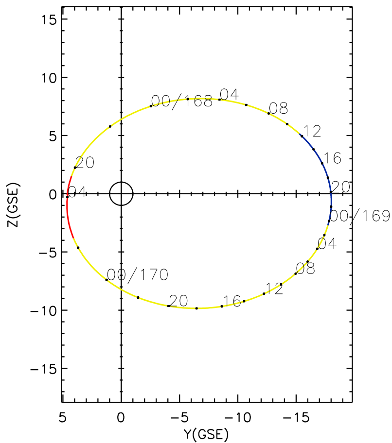
CLUSTER 2 orbit 2004 167 (06/15) 19:01 UT to 2004 170 (06/18) 04:06 UT
