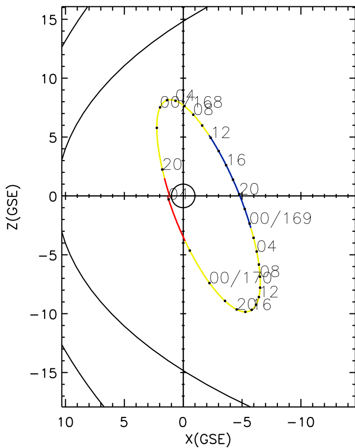
CLUSTER 2 orbit 2004 167 (06/15) 19:01 UT to 2004 170 (06/18) 04:06 UT
