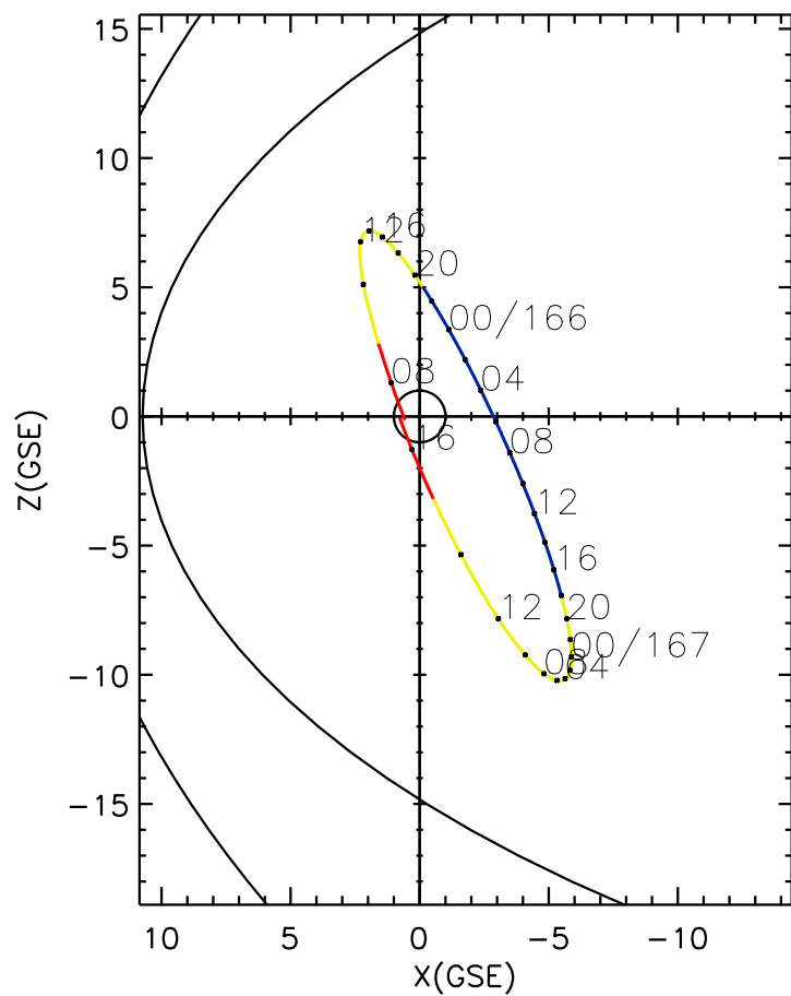
CLUSTER 2 orbit 2004 165 (06/13) 07:25 UT to 2004 167 (06/15) 16:30 UT
