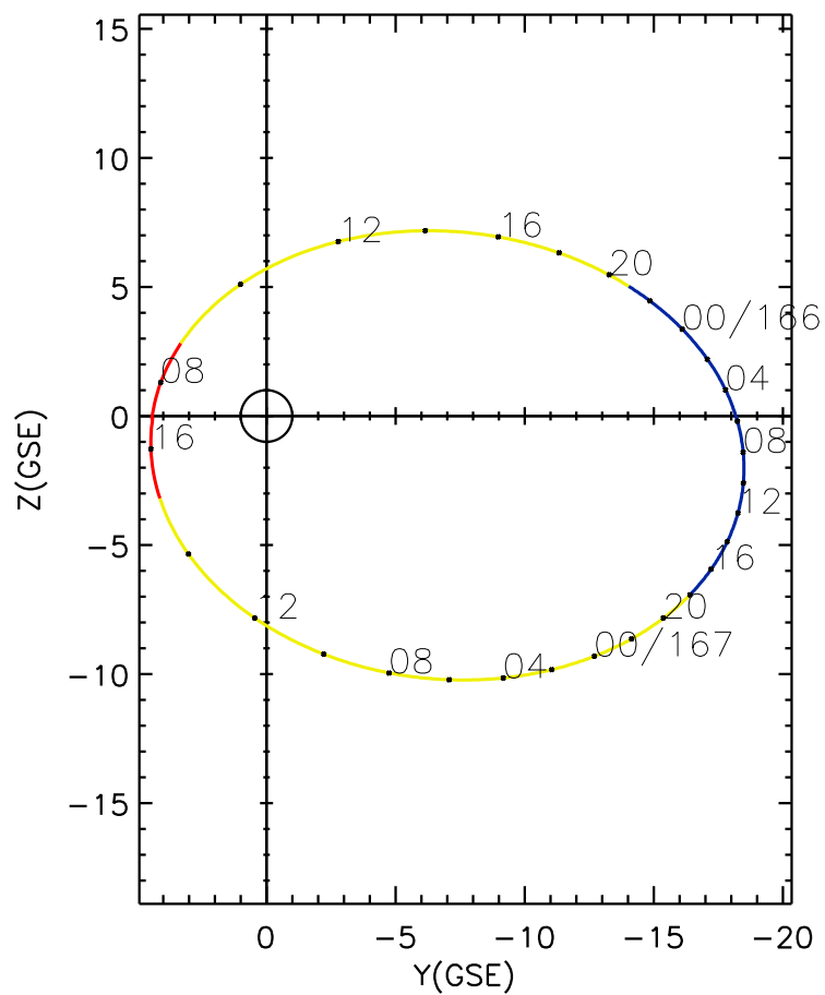
CLUSTER 2 orbit 2004 165 (06/13) 07:25 UT to 2004 167 (06/15) 16:30 UT
