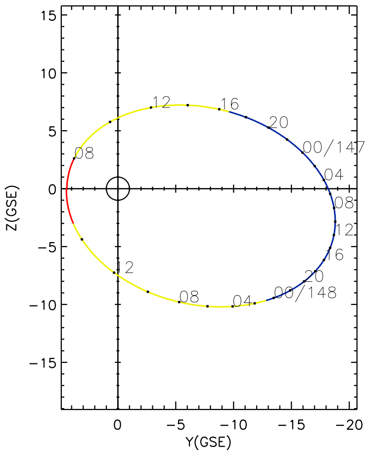
CLUSTER 2 orbit 2004 146 (05/25) 06:51 UT to 2004 148 (05/27) 15:56 UT
