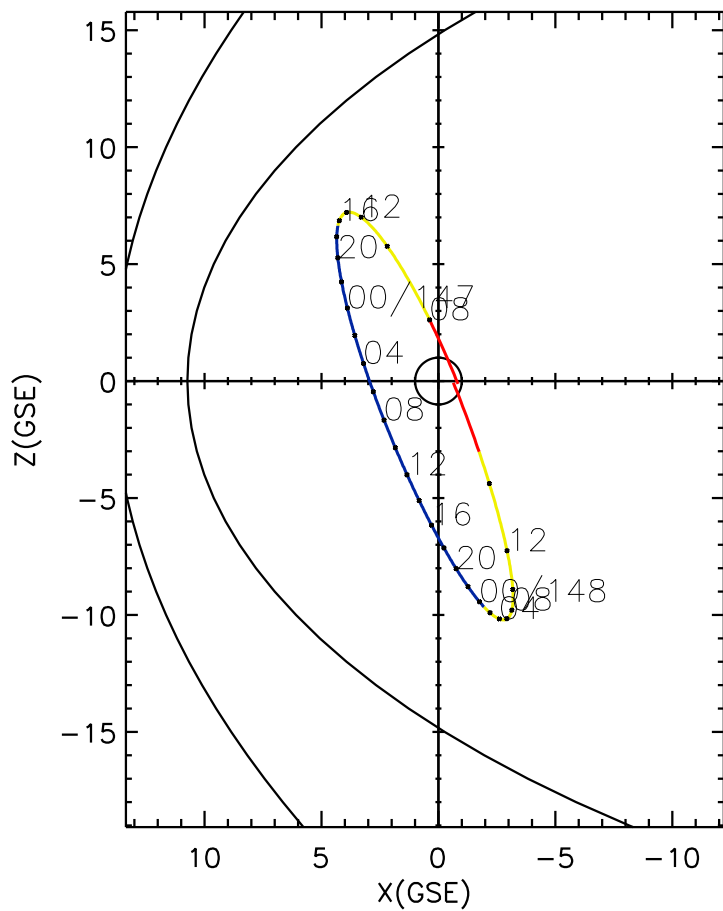
CLUSTER 2 orbit 2004 146 (05/25) 06:51 UT to 2004 148 (05/27) 15:56 UT
