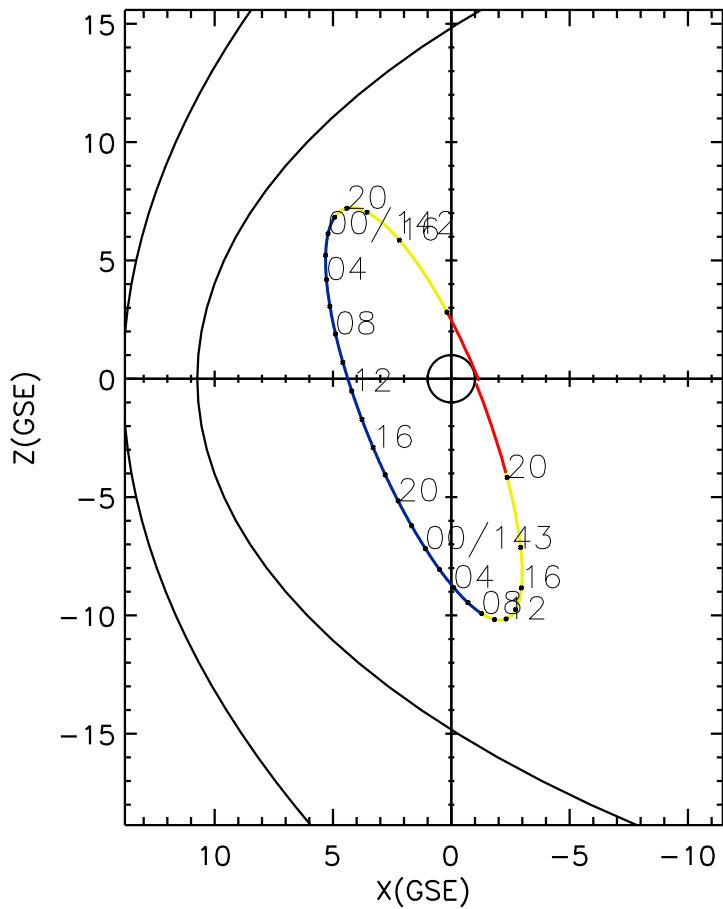
CLUSTER 2 orbit 2004 141 (05/20) 12:46 UT to 2004 143 (05/22) 21:46 UT
