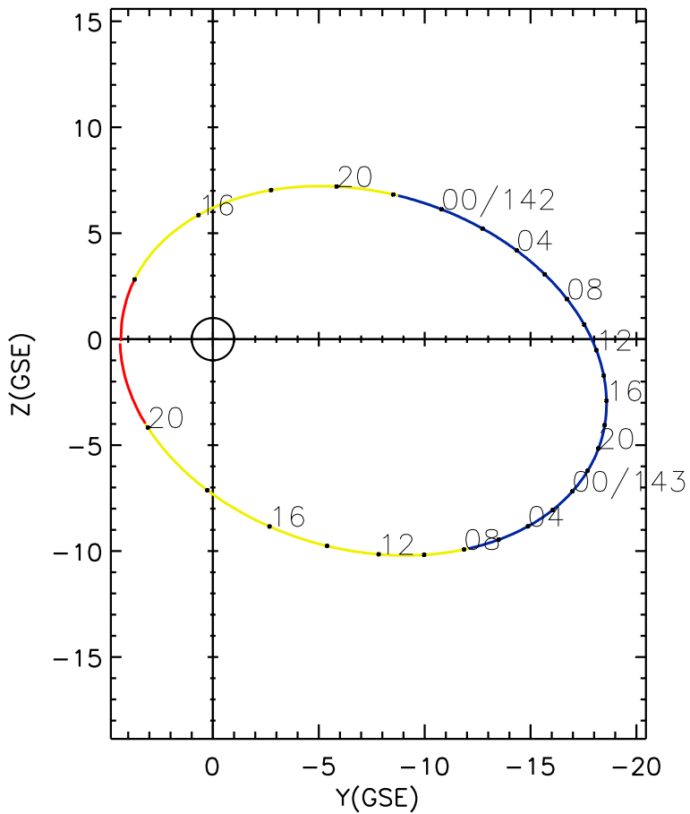
CLUSTER 2 orbit 2004 141 (05/20) 12:46 UT to 2004 143 (05/22) 21:46 UT
