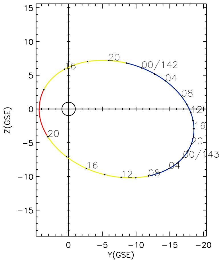
CLUSTER 2 orbit 2004 141 (05/20) 12:41 UT to 2004 143 (05/22) 21:46 UT
