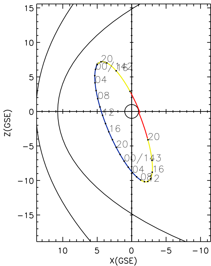
CLUSTER 2 orbit 2004 141 (05/20) 12:41 UT to 2004 143 (05/22) 21:46 UT
