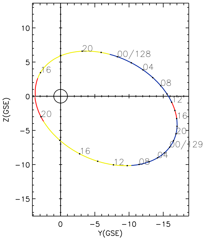
CLUSTER 2 orbit 2004 127 (05/06) 14:31 UT to 2004 129 (05/08) 21:11 UT
