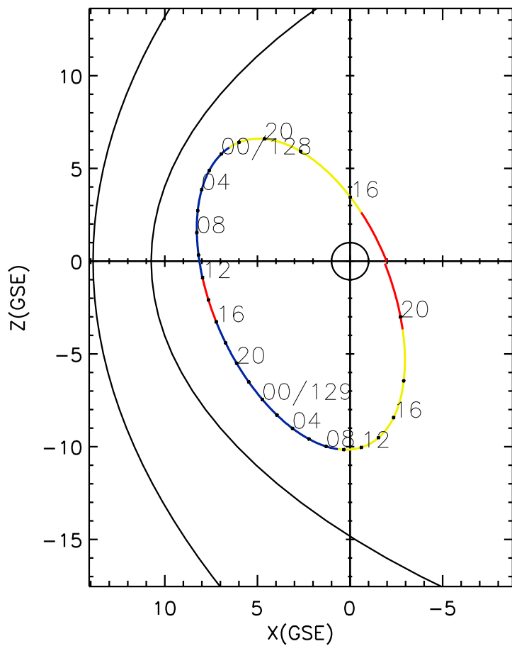
CLUSTER 2 orbit 2004 127 (05/06) 14:31 UT to 2004 129 (05/08) 21:11 UT
