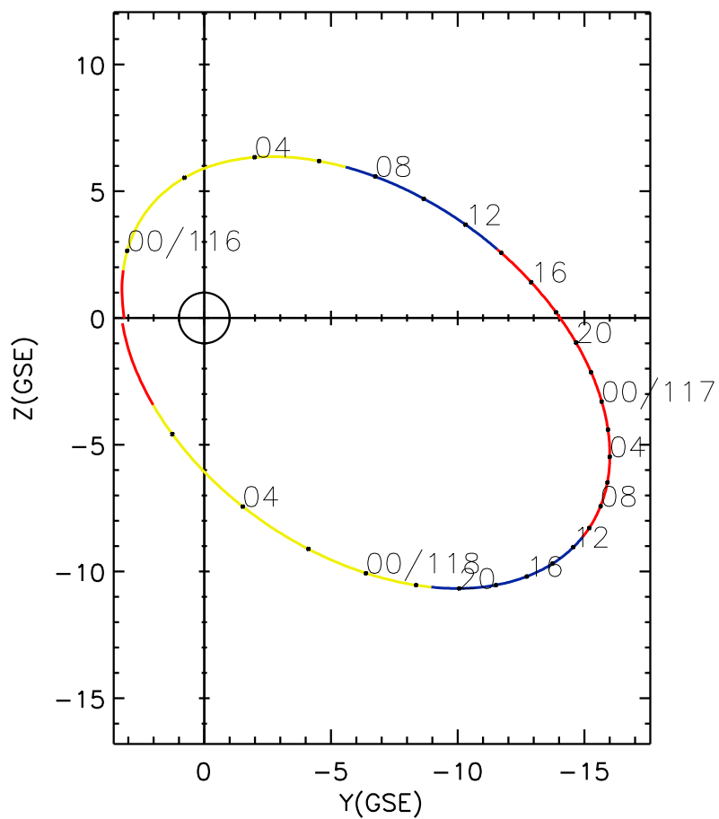
CLUSTER 2 orbit 2004 115 (04/24) 22:55 UT to 2004 118 (04/27) 07:55 UT
