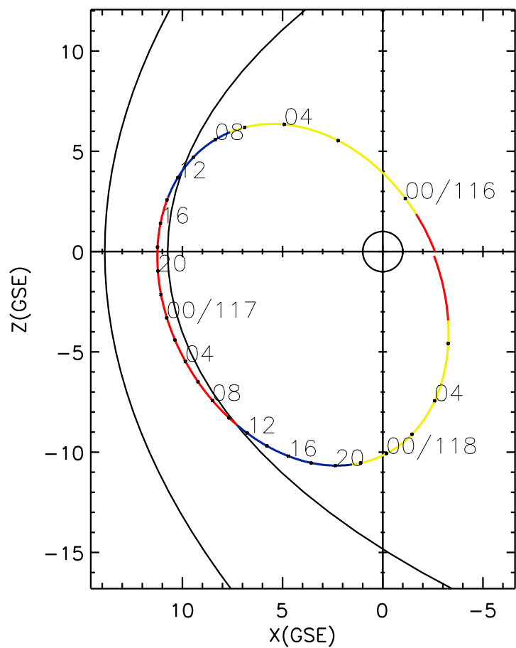
CLUSTER 2 orbit 2004 115 (04/24) 22:55 UT to 2004 118 (04/27) 07:55 UT
