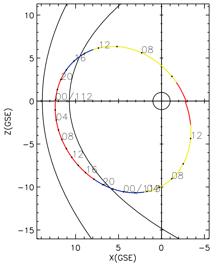
CLUSTER 2 orbit 2004 111 (04/20) 04:46 UT to 2004 113 (04/22) 13:50 UT
