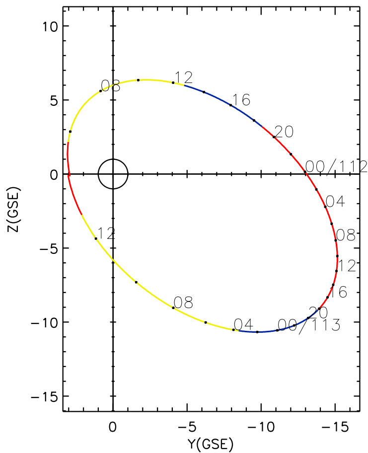
CLUSTER 2 orbit 2004 111 (04/20) 04:46 UT to 2004 113 (04/22) 13:50 UT
