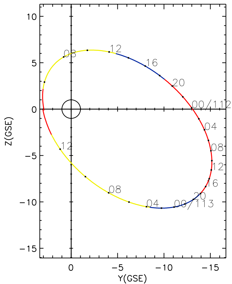
CLUSTER 2 orbit 2004 111 (04/20) 04:45 UT to 2004 113 (04/22) 13:50 UT
