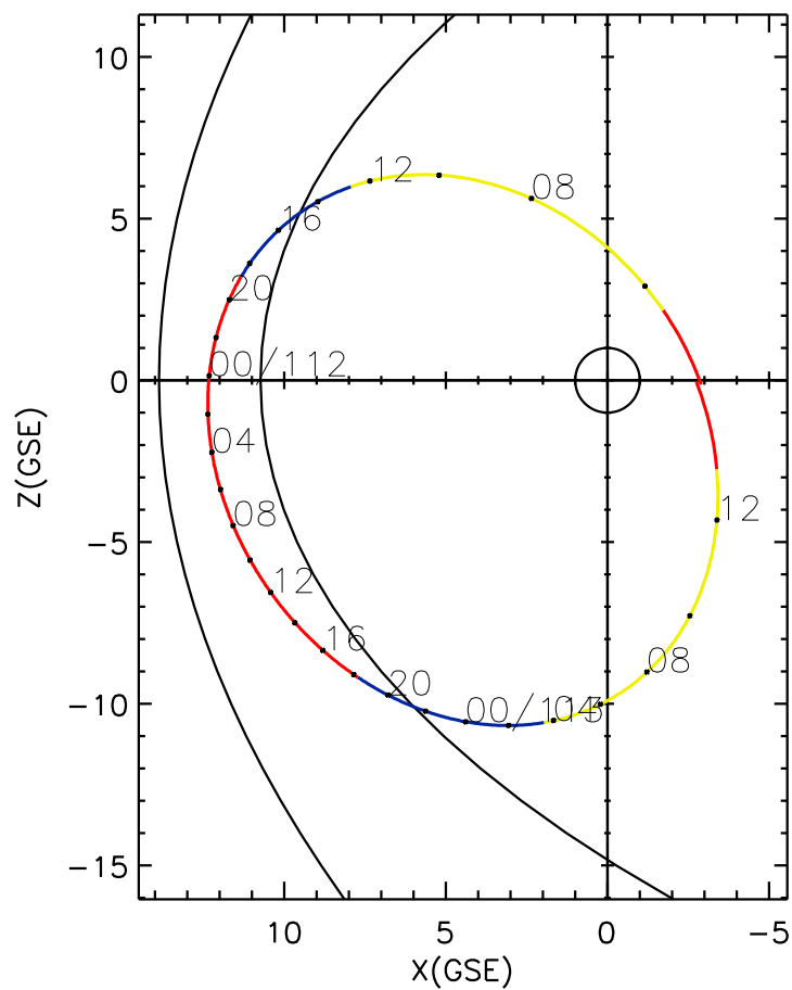
CLUSTER 2 orbit 2004 111 (04/20) 04:45 UT to 2004 113 (04/22) 13:50 UT
