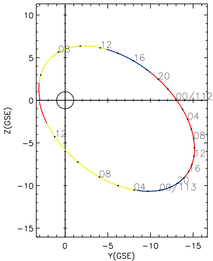
CLUSTER 2 orbit 2004 111 (04/20) 04:45 UT to 2004 113 (04/22) 13:45 UT
