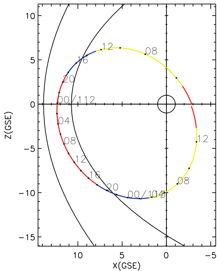
CLUSTER 2 orbit 2004 111 (04/20) 04:45 UT to 2004 113 (04/22) 13:45 UT
