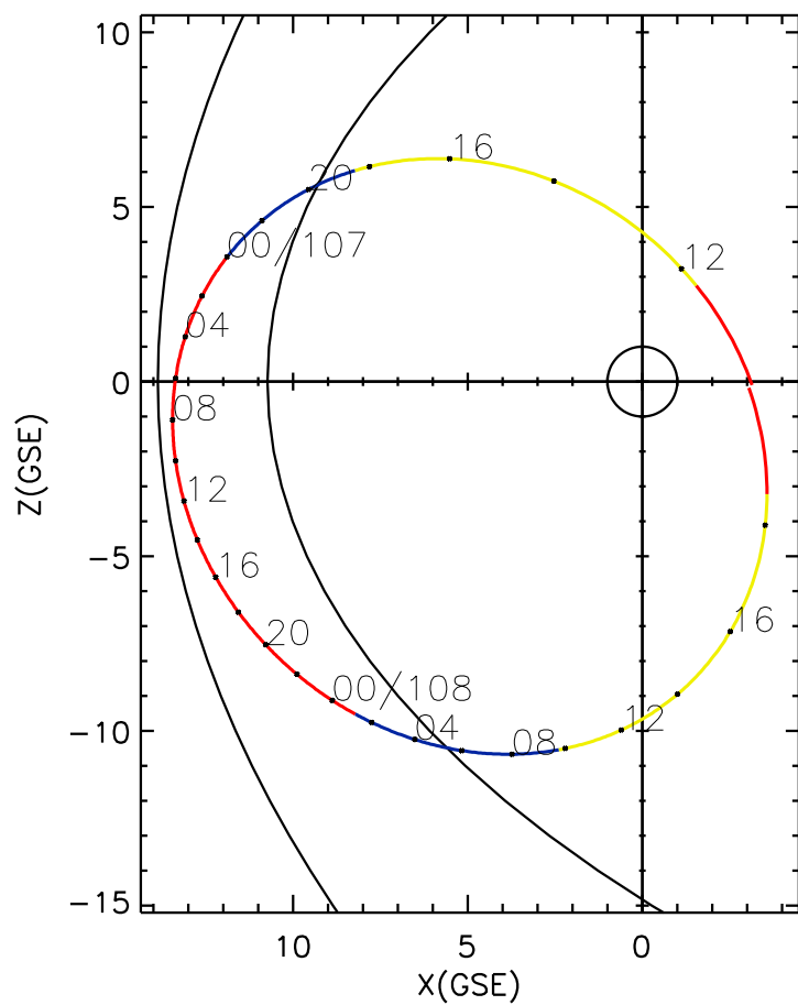
CLUSTER 2 orbit 2004 106 (04/15) 10:36 UT to 2004 108 (04/17) 19:41 UT
