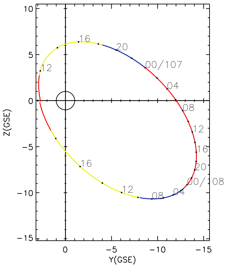
CLUSTER 2 orbit 2004 106 (04/15) 10:36 UT to 2004 108 (04/17) 19:41 UT
