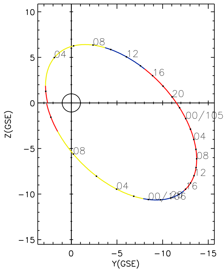
CLUSTER 2 orbit 2004 104 (04/13) 01:30 UT to 2004 106 (04/15) 10:35 UT
