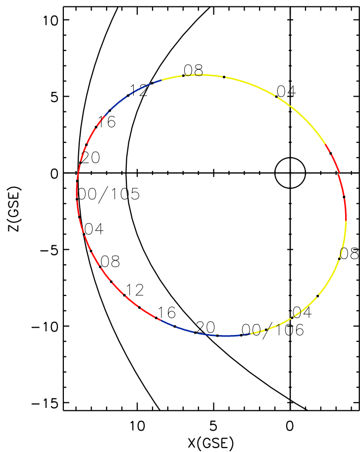
CLUSTER 2 orbit 2004 104 (04/13) 01:30 UT to 2004 106 (04/15) 10:35 UT
