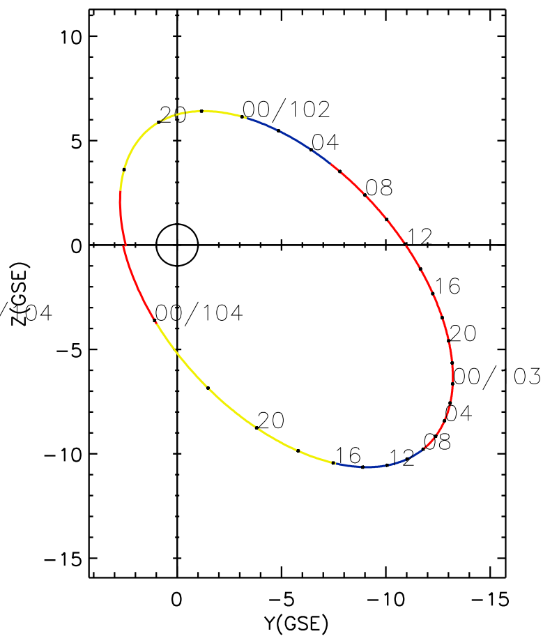
CLUSTER 2 orbit 2004 101 (04/10) 16:25 UT to 2004 104 (04/13) 01:30 UT
