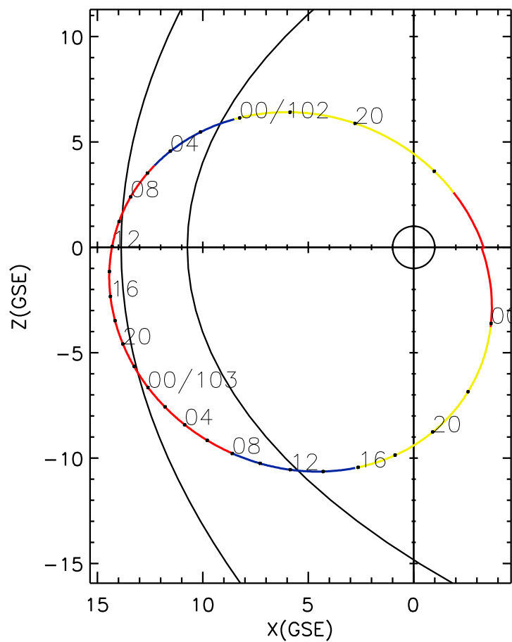
CLUSTER 2 orbit 2004 101 (04/10) 16:25 UT to 2004 104 (04/13) 01:30 UT
