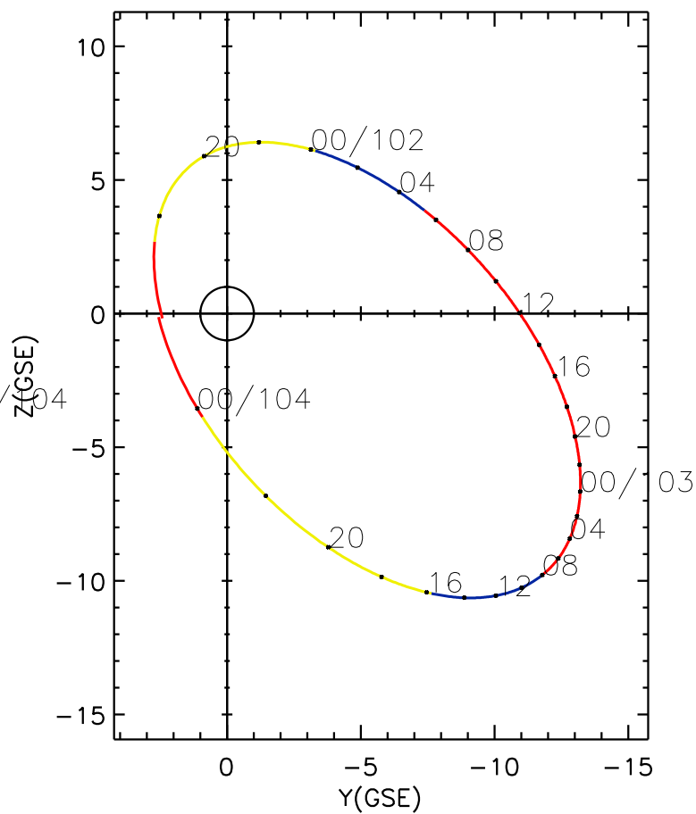
CLUSTER 2 orbit 2004 101 (04/10) 16:21 UT to 2004 104 (04/13) 01:26 UT
