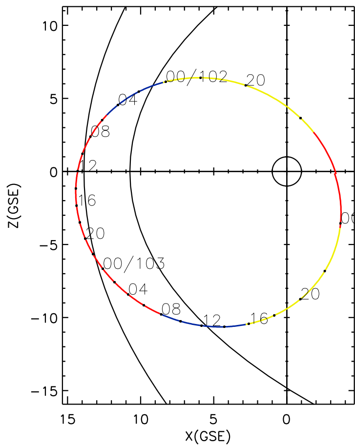
CLUSTER 2 orbit 2004 101 (04/10) 16:21 UT to 2004 104 (04/13) 01:26 UT
