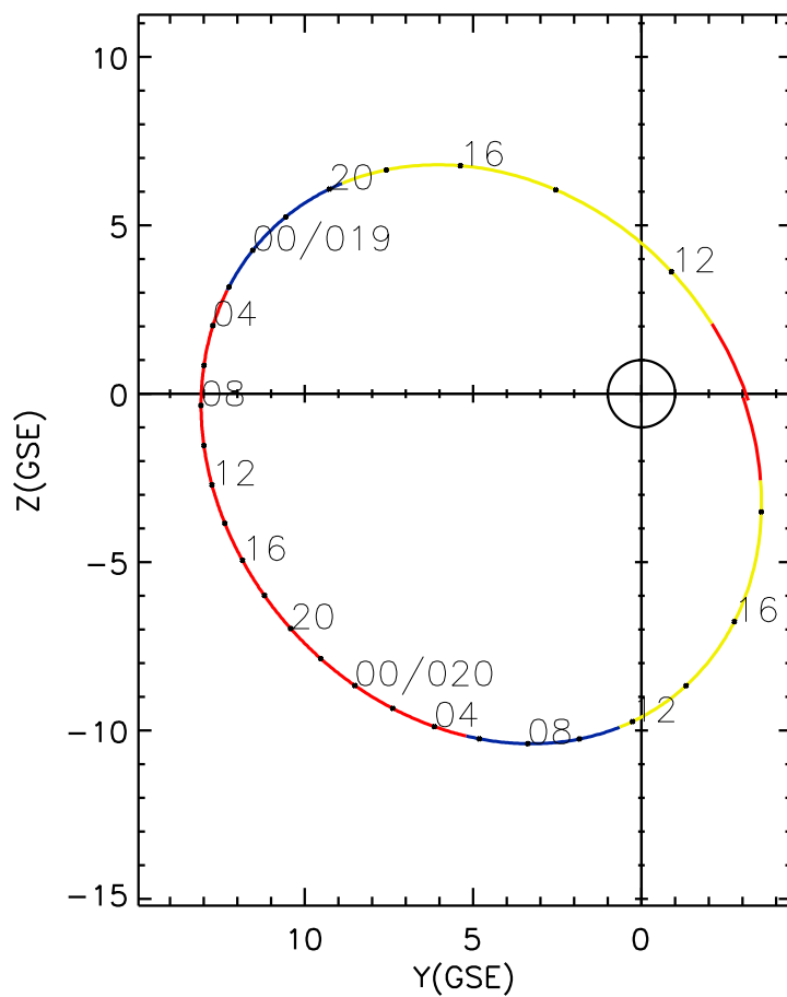
CLUSTER 2 orbit 2004 018 (01/18) 10:20 UT to 2004 020 (01/20) 19:25 UT
