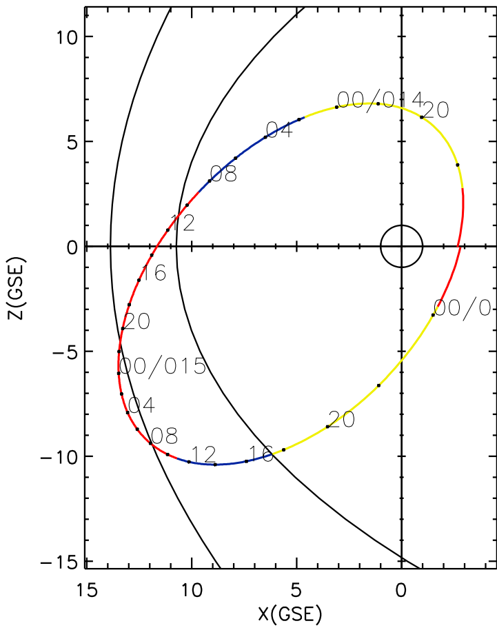
CLUSTER 2 orbit 2004 013 (01/13) 16:16 UT to 2004 016 (01/16) 01:21 UT
