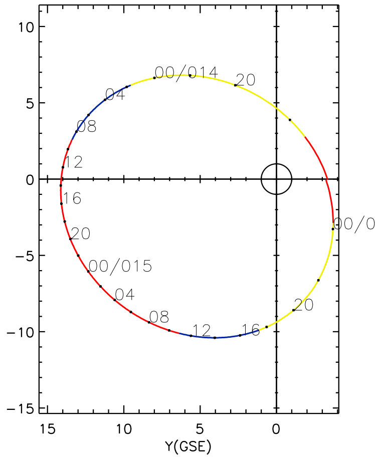
CLUSTER 2 orbit 2004 013 (01/13) 16:16 UT to 2004 016 (01/16) 01:21 UT
