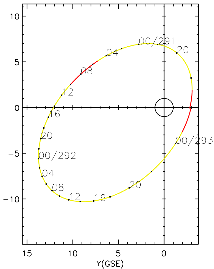
CLUSTER 2 orbit 2003 290 (10/17) 16:35 UT to 2003 293 (10/20) 01:40 UT
