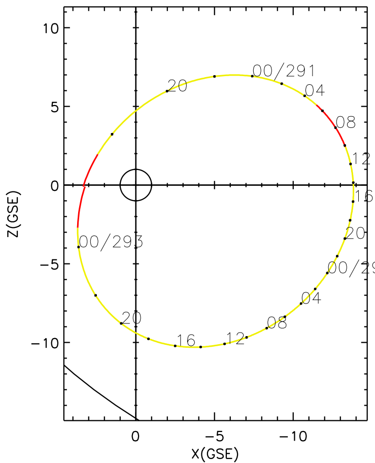
CLUSTER 2 orbit 2003 290 (10/17) 16:35 UT to 2003 293 (10/20) 01:40 UT
