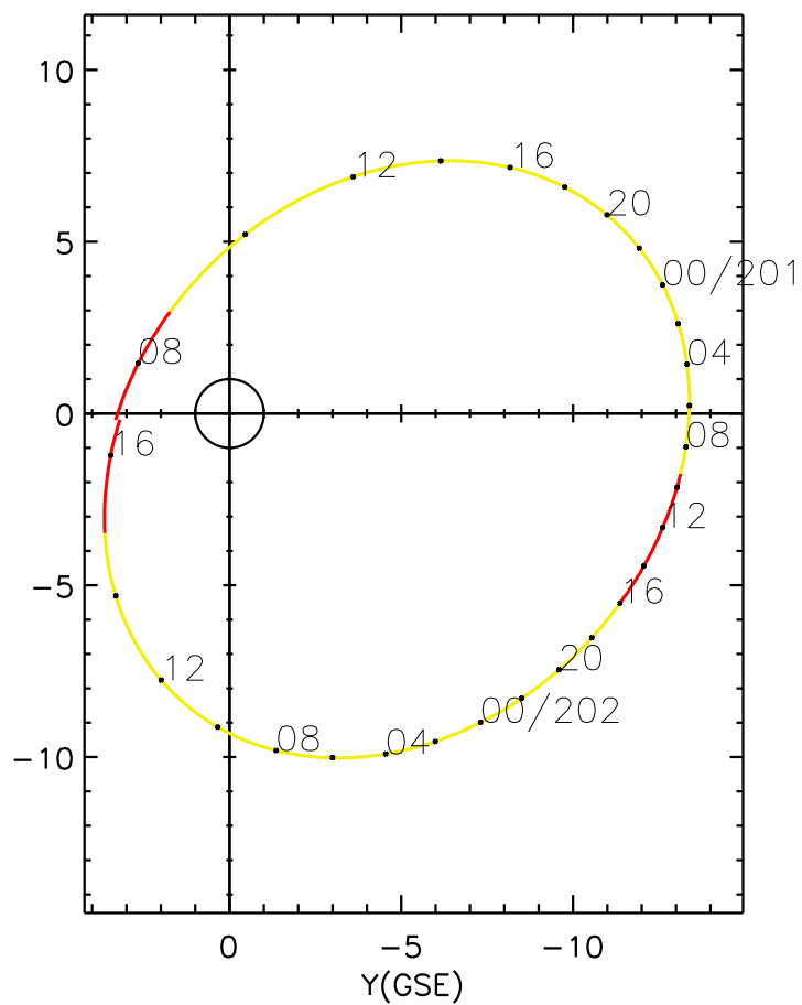
CLUSTER 2 orbit 2003 200 (07/19) 07:20 UT to 2003 202 (07/21) 16:25 UT
