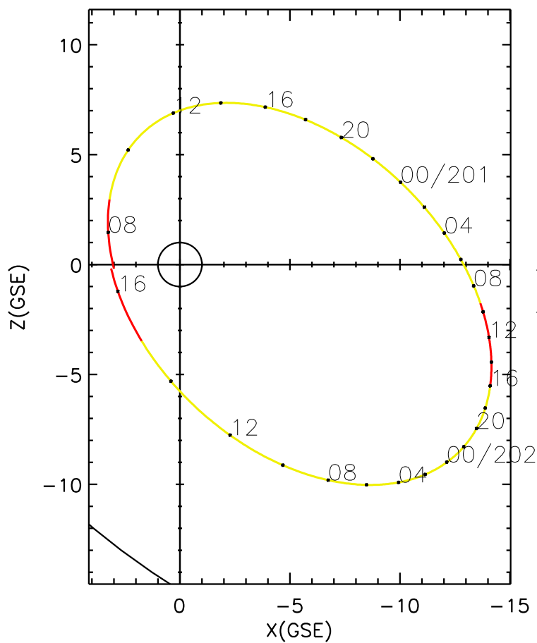
CLUSTER 2 orbit 2003 200 (07/19) 07:20 UT to 2003 202 (07/21) 16:25 UT
