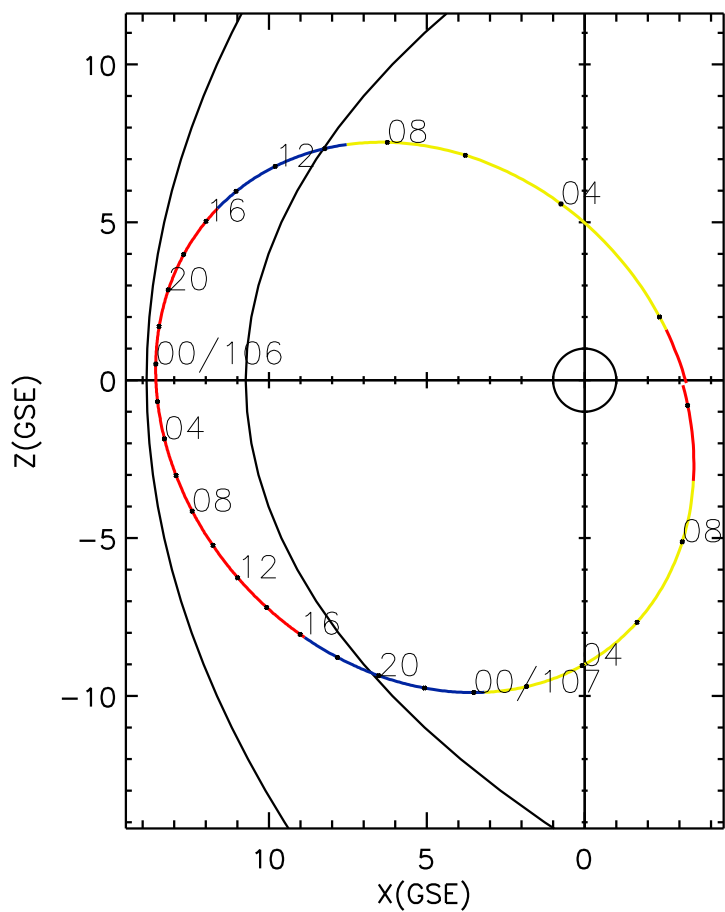
CLUSTER 2 orbit 2003 105 (04/15) 01:10 UT to 2003 107 (04/17) 10:15 UT
