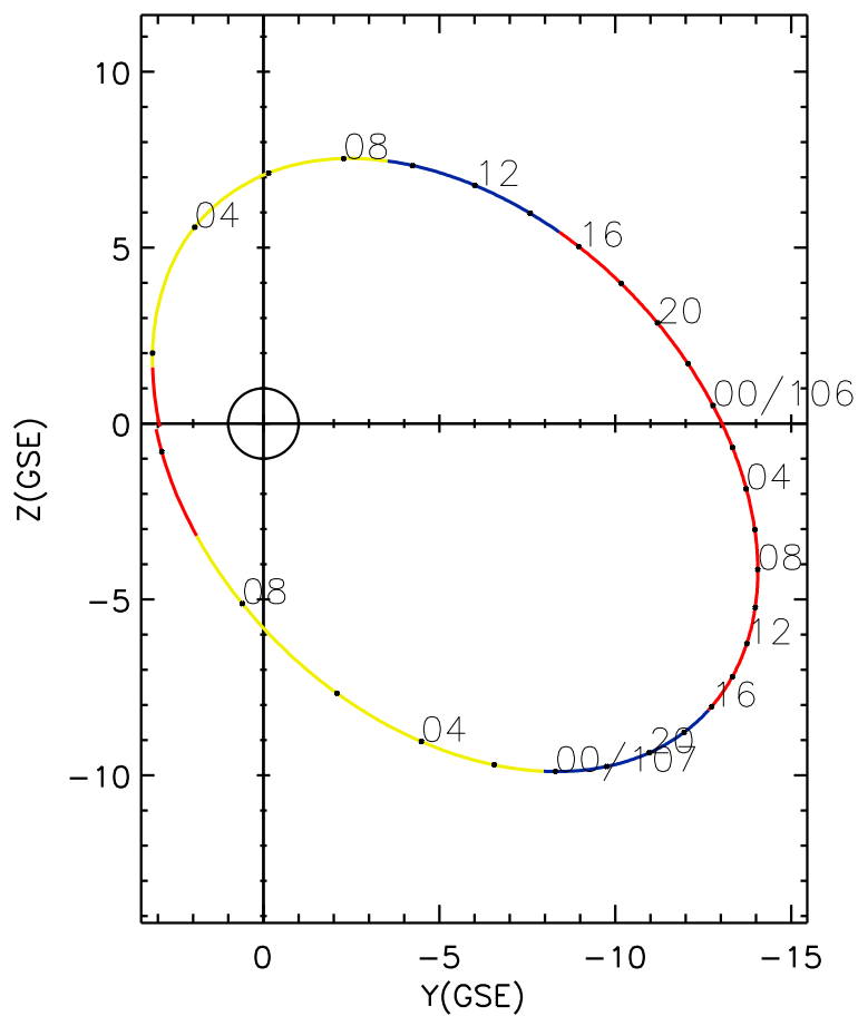
CLUSTER 2 orbit 2003 105 (04/15) 01:10 UT to 2003 107 (04/17) 10:15 UT
