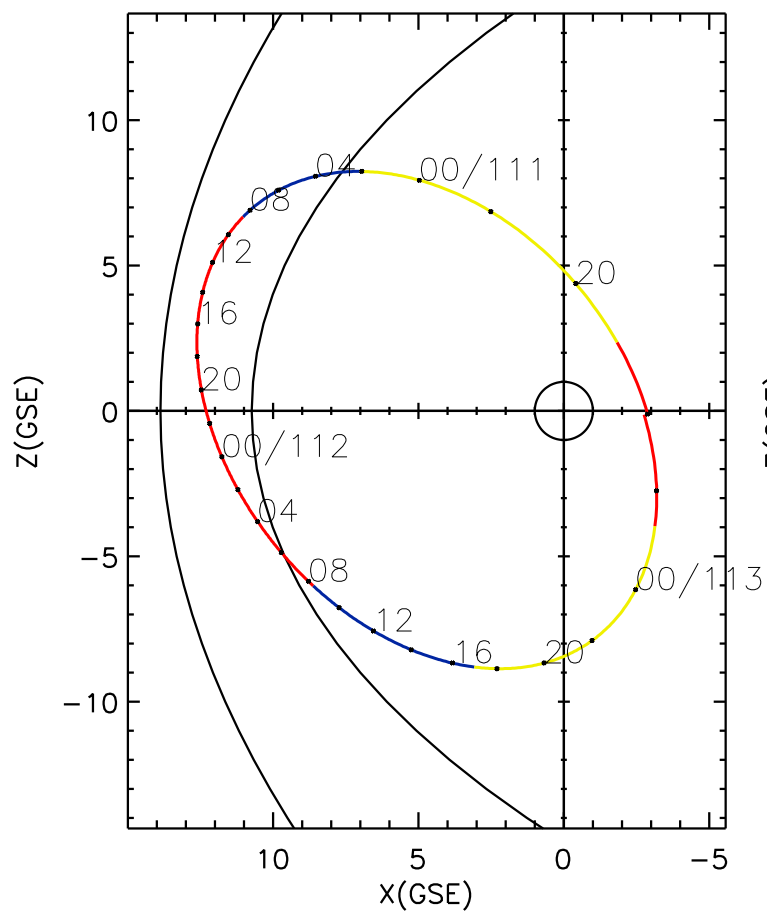
CLUSTER 2 orbit 2002 110 (04/20) 18:00 UT to 2002 113 (04/23) 03:05 UT
