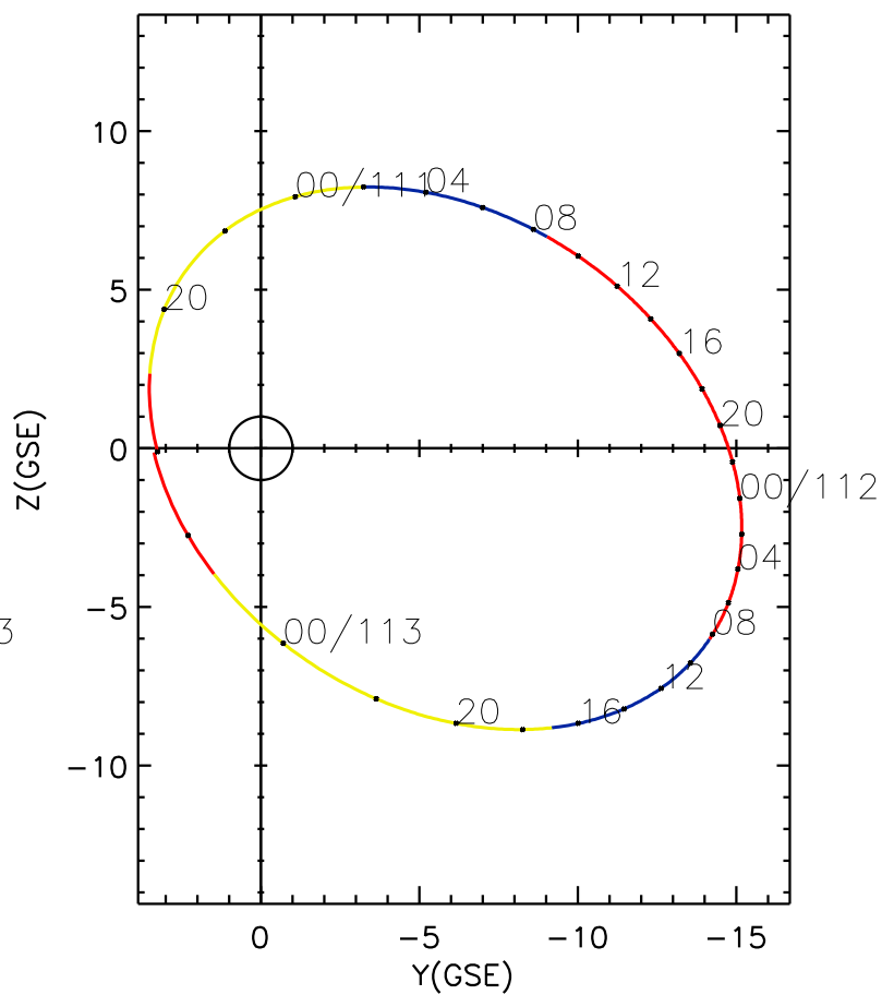
CLUSTER 2 orbit 2002 110 (04/20) 18:00 UT to 2002 113 (04/23) 03:05 UT
