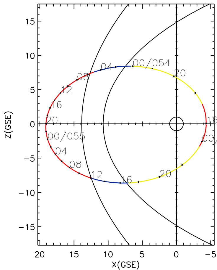
CLUSTER 2 orbit 2002 053 (02/22) 15:55 UT to 2002 056 (02/25) 01:00 UT
