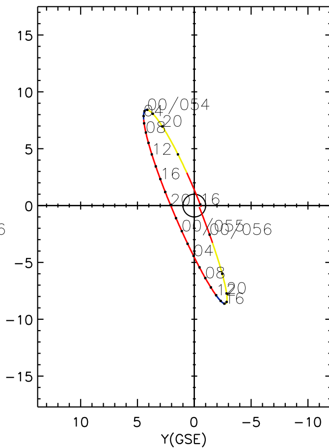
CLUSTER 2 orbit 2002 053 (02/22) 15:55 UT to 2002 056 (02/25) 01:00 UT
