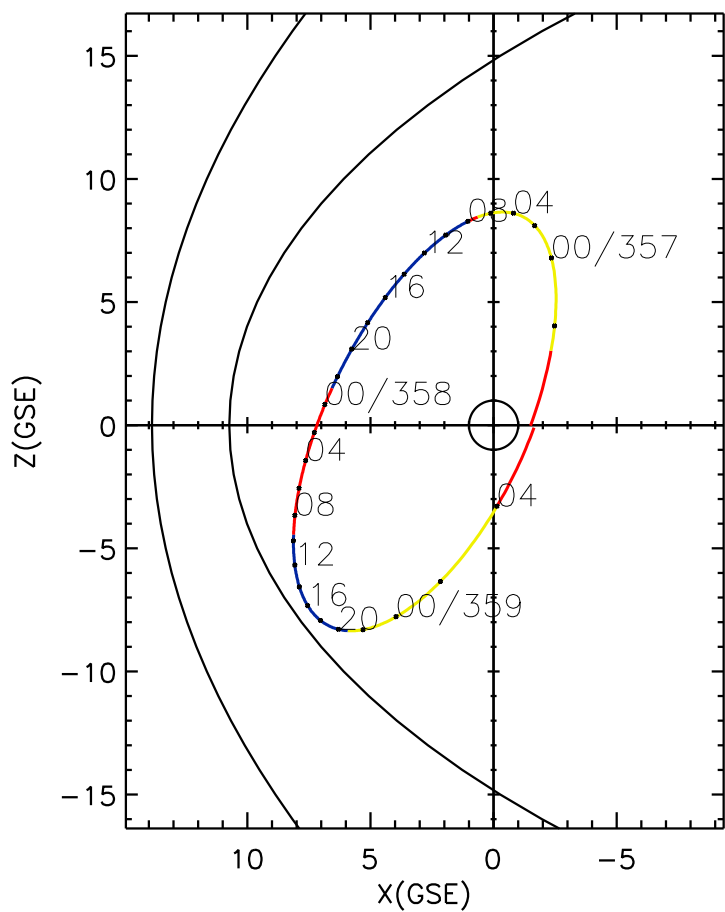
CLUSTER 2 orbit 2001 356 (12/22) 20:15 UT to 2001 359 (12/25) 05:20 UT
