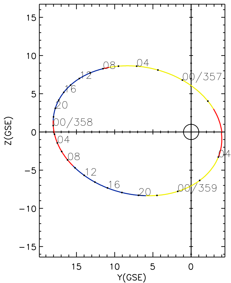
CLUSTER 2 orbit 2001 356 (12/22) 20:15 UT to 2001 359 (12/25) 05:20 UT
