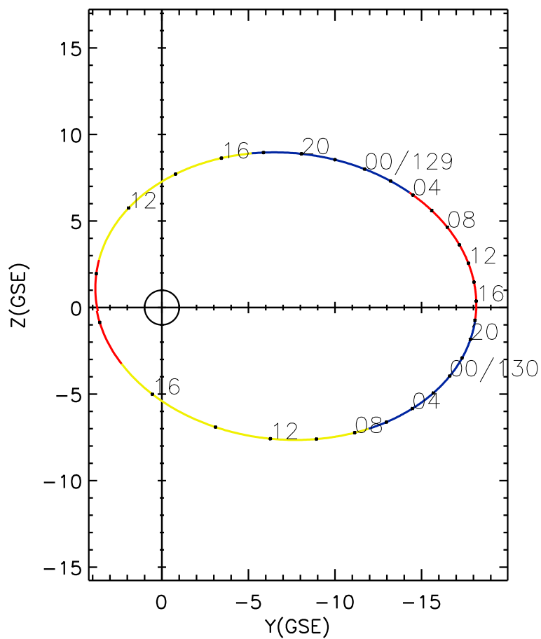
CLUSTER 2 orbit 2001 128 (05/08) 09:10 UT to 2001 130 (05/10) 18:15 UT
