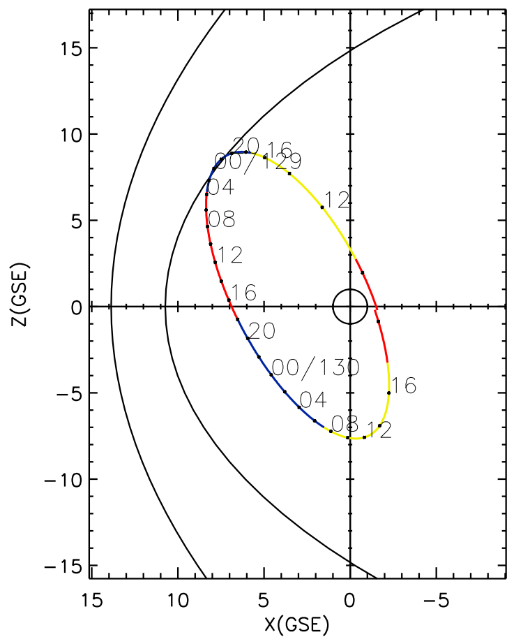
CLUSTER 2 orbit 2001 128 (05/08) 09:10 UT to 2001 130 (05/10) 18:15 UT
