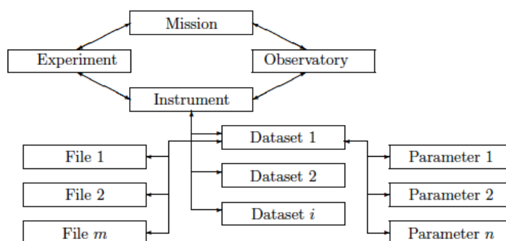
Figure 1: The CAA hierarchy of concepts.
