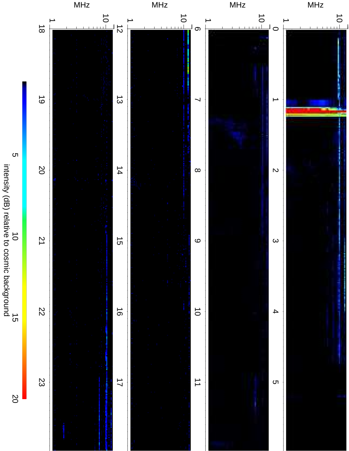
Wind Waves RAD2 receiver: 2019/09/23
