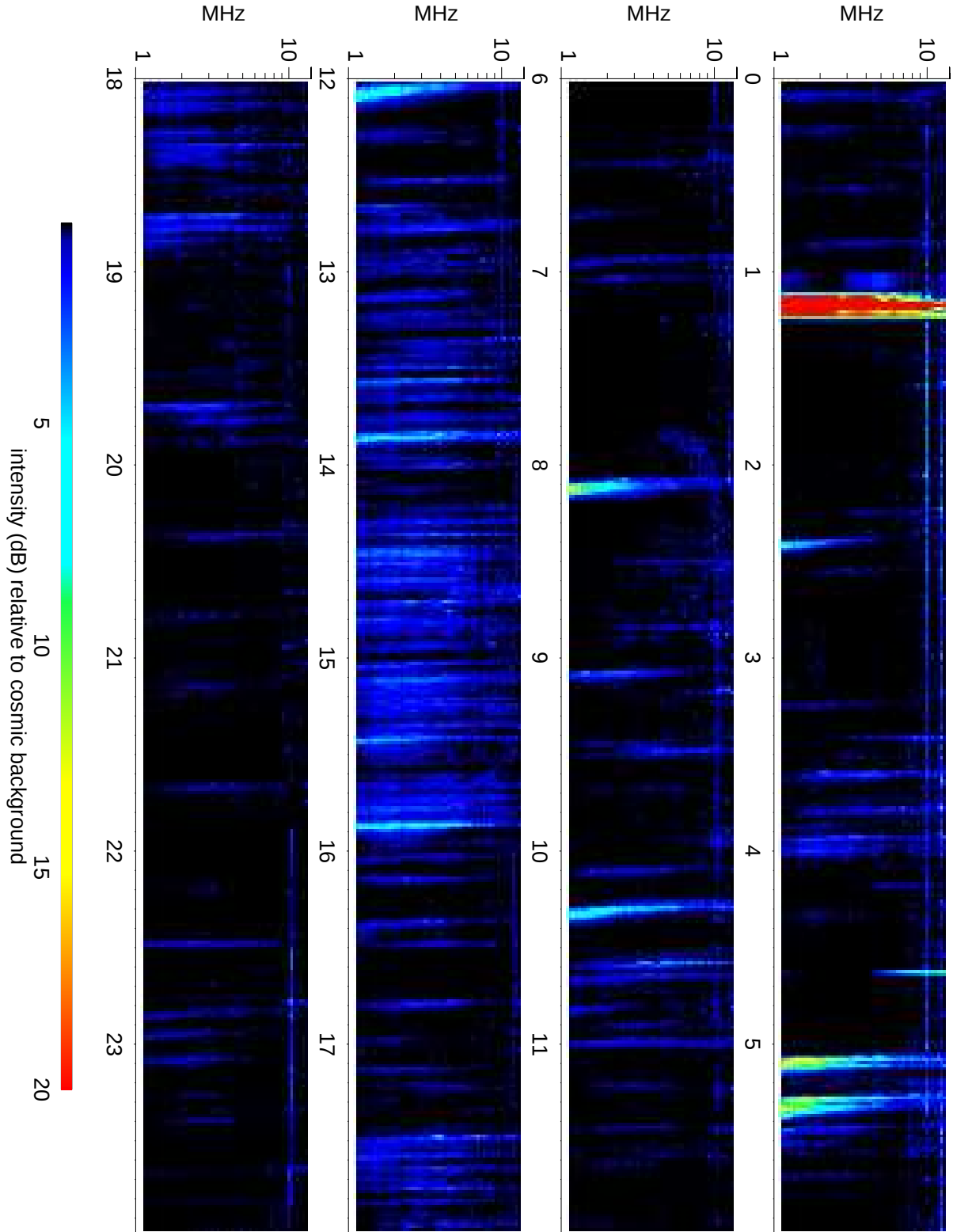
Wind Waves RAD2 receiver: 2019/04/14
