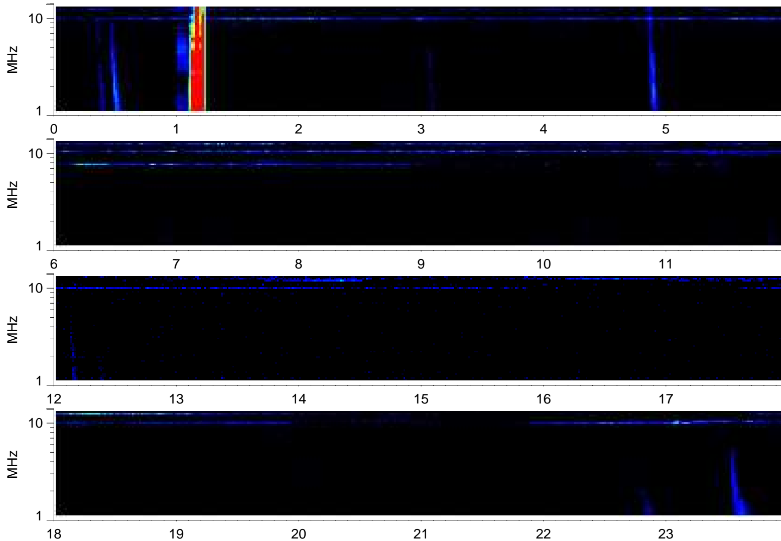
Wind Waves RAD2 receiver: 2016/06/24
