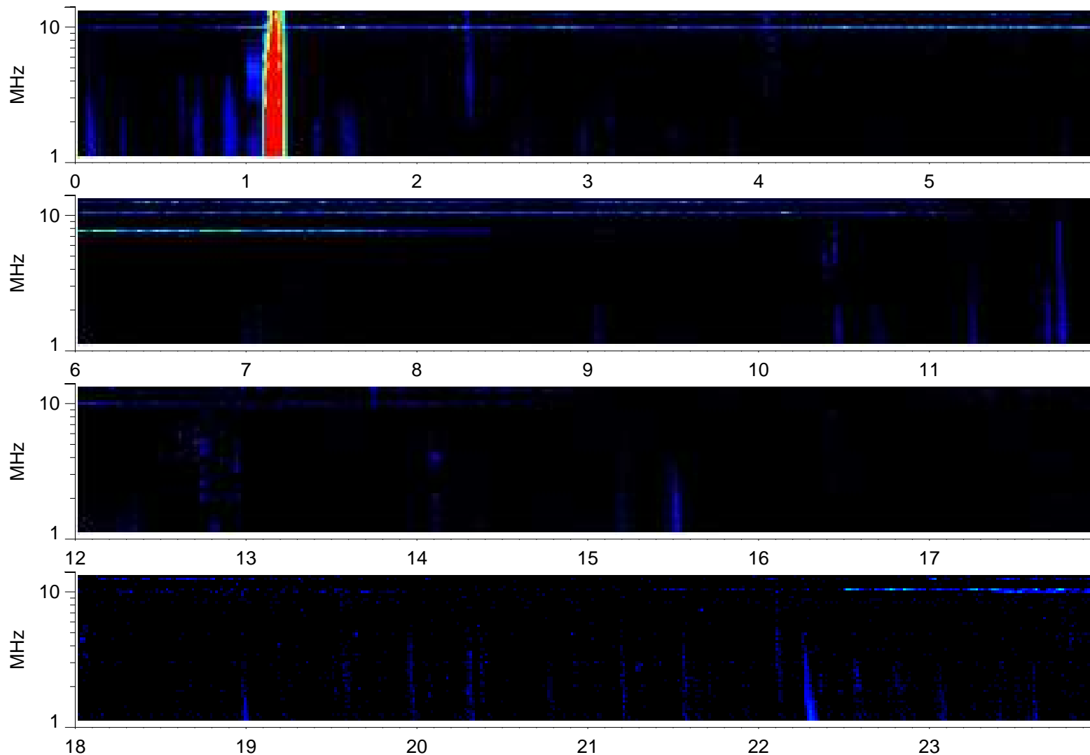
Wind Waves RAD2 receiver: 2016/06/18
