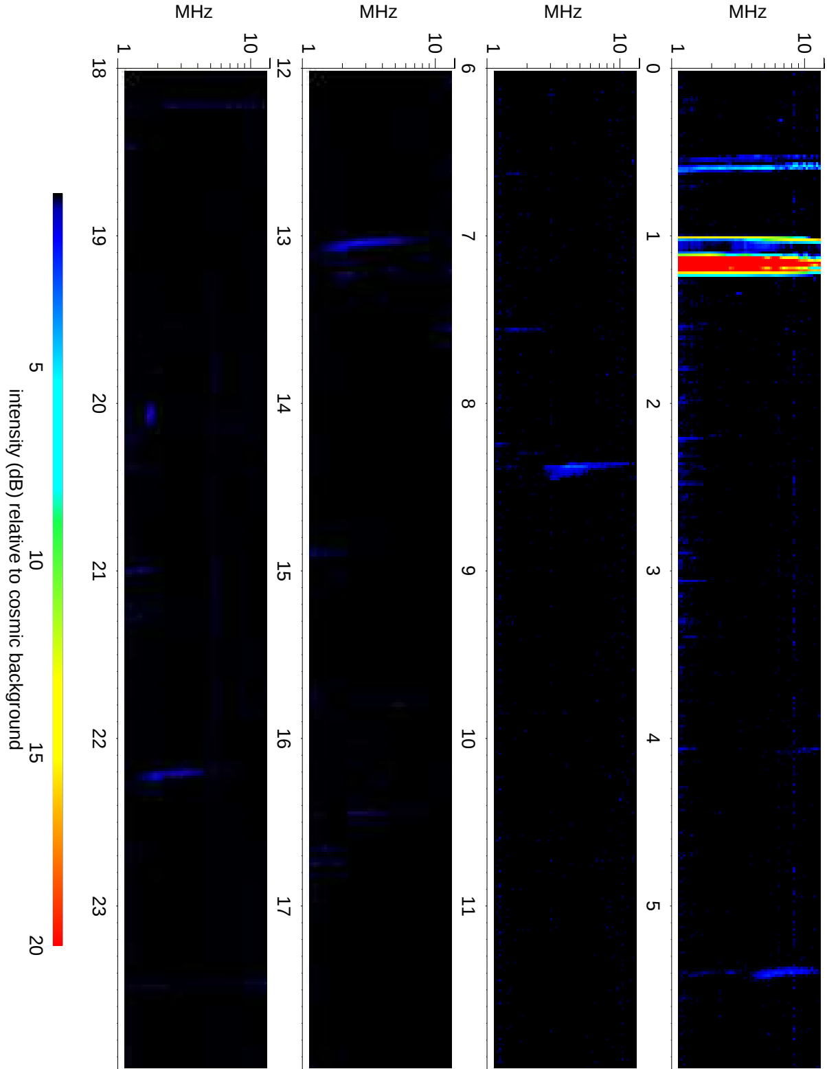
Wind Waves RAD2 receiver: 2012/03/08
