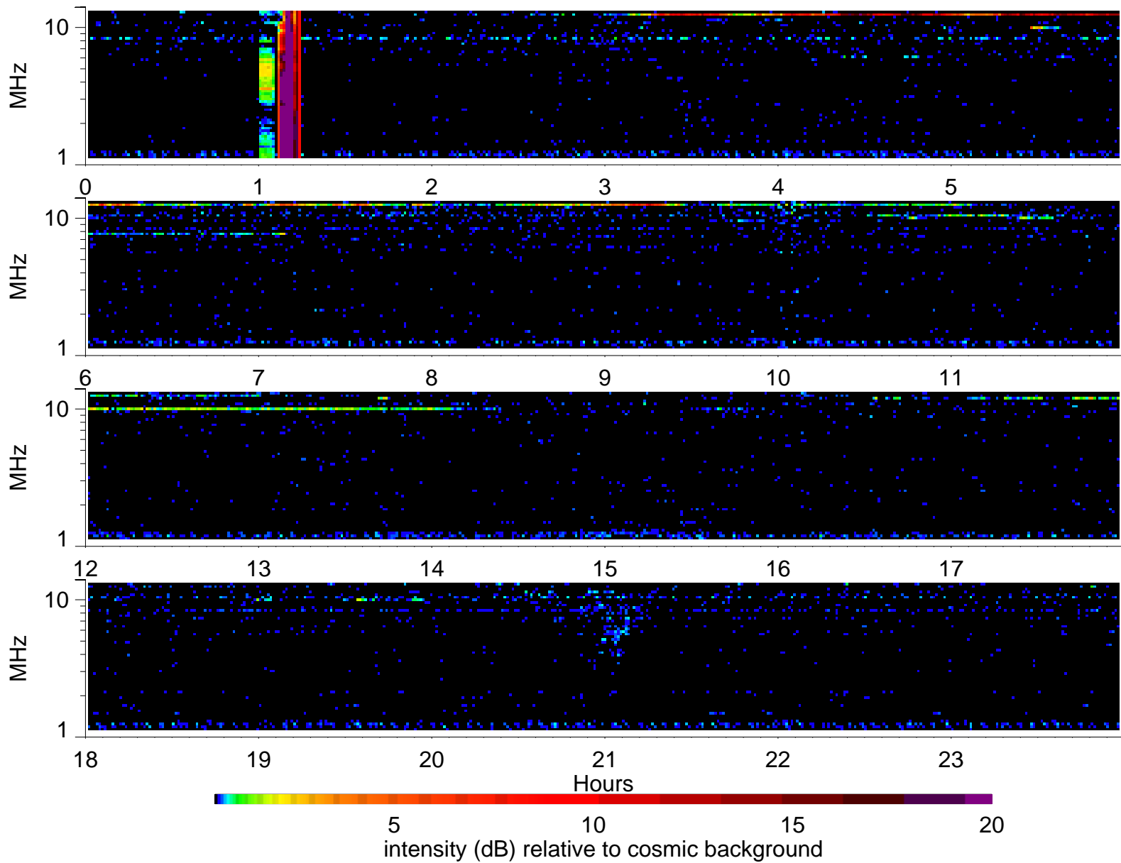
Wind Waves RAD2 receiver: 2007/11/24
