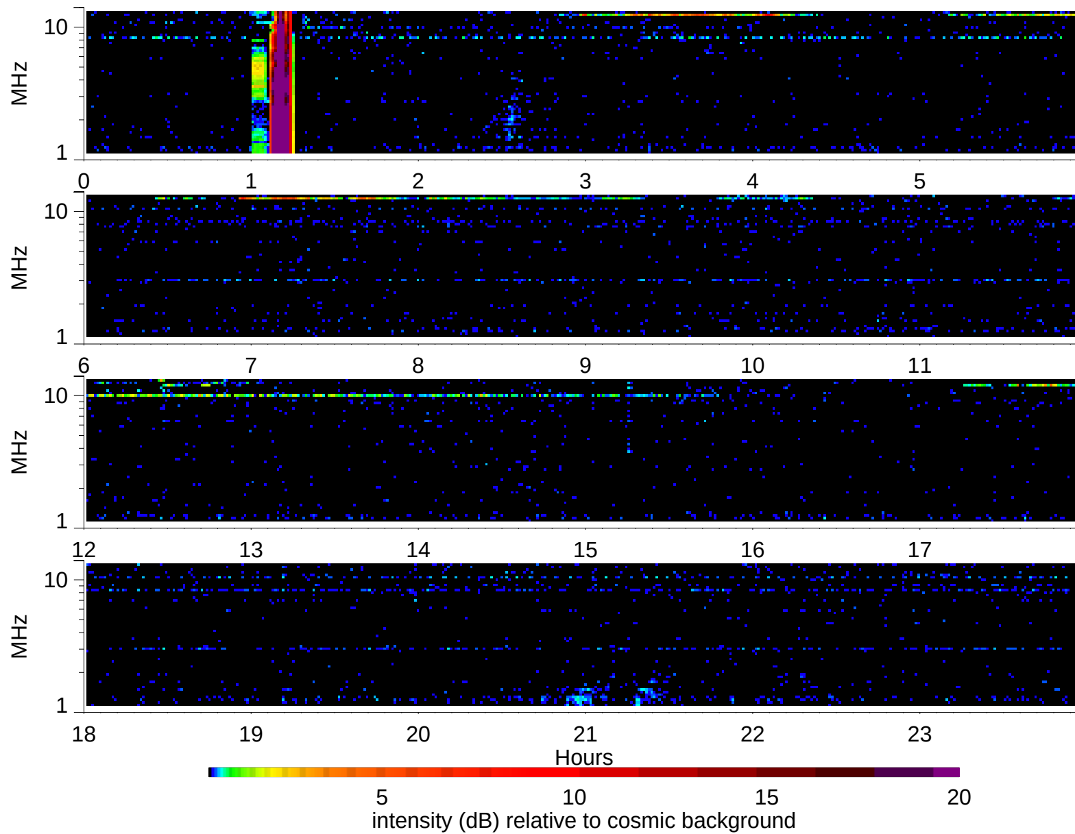
Wind Waves RAD2 receiver: 2007/10/31
