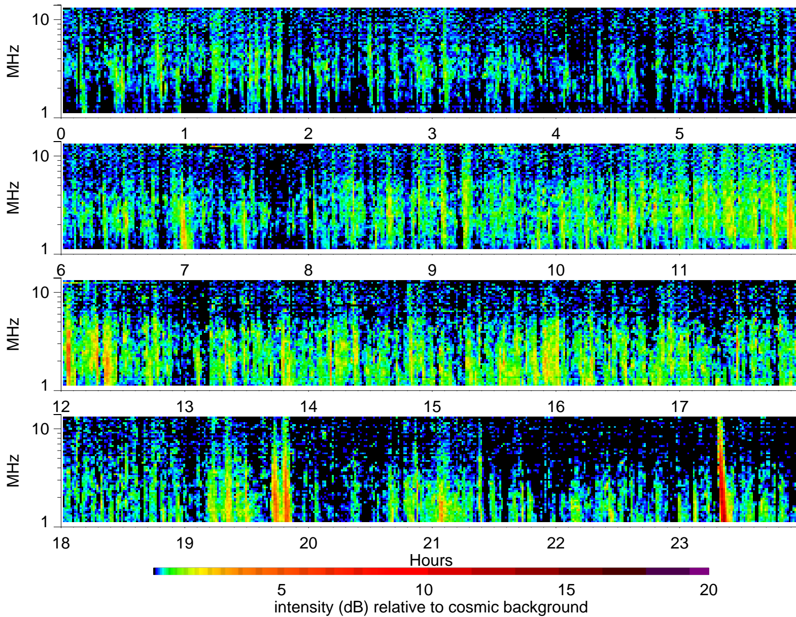
Wind Waves RAD2 receiver: 2005/11/19
