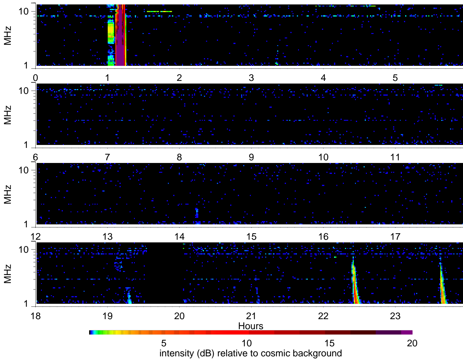
Wind Waves RAD2 receiver: 2005/11/10
