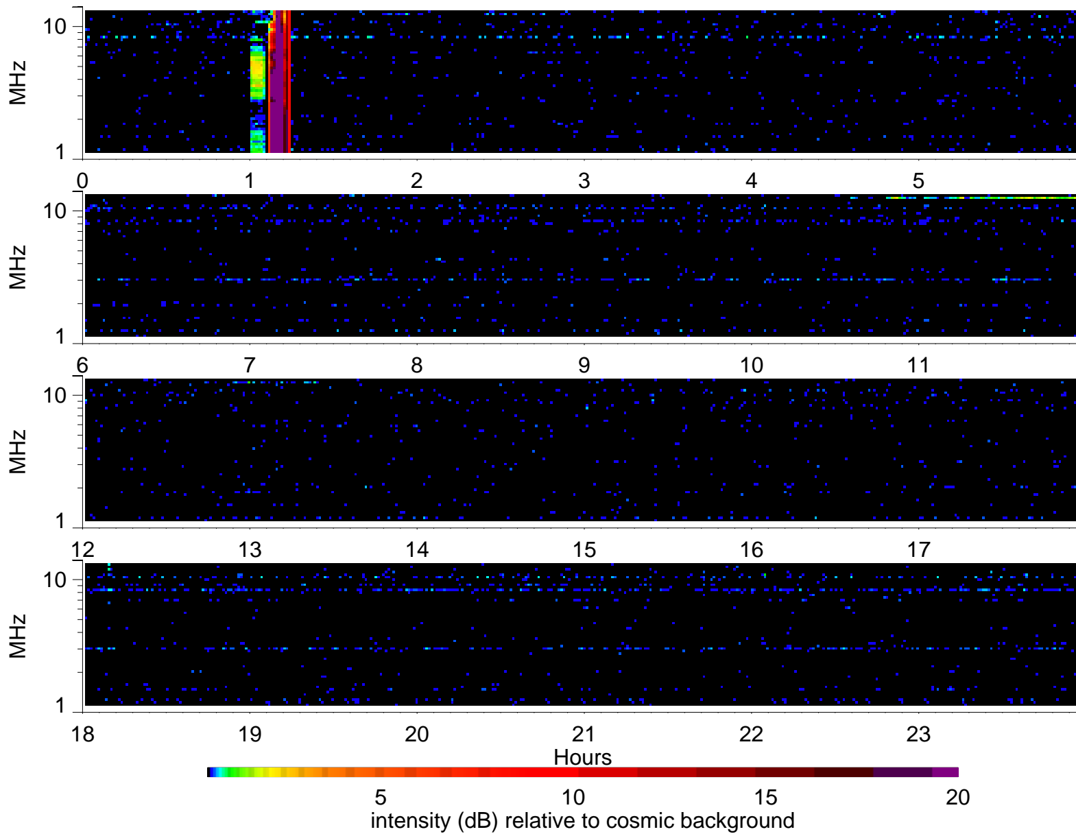
Wind Waves RAD2 receiver: 2005/10/19
