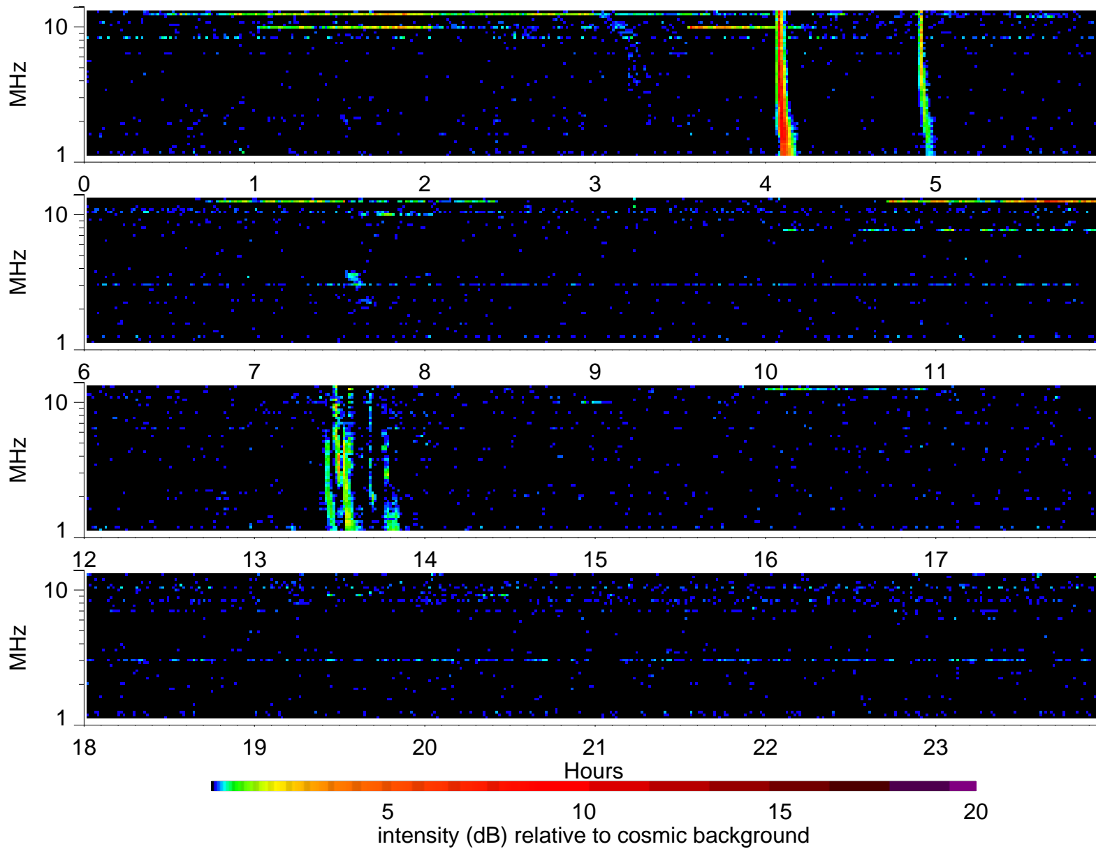
Wind Waves RAD2 receiver: 2005/10/6
