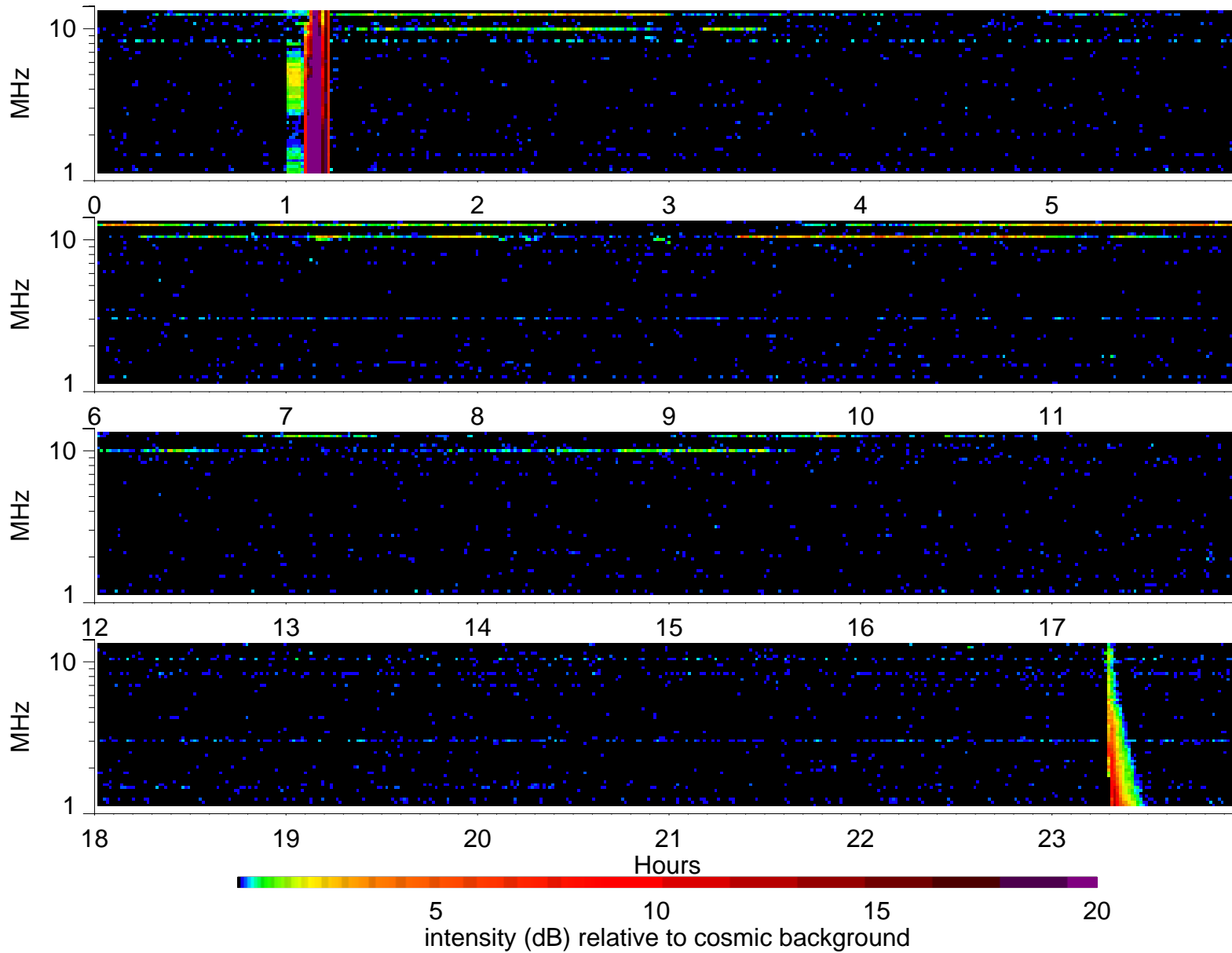
Wind Waves RAD2 receiver: 2005/10/1
