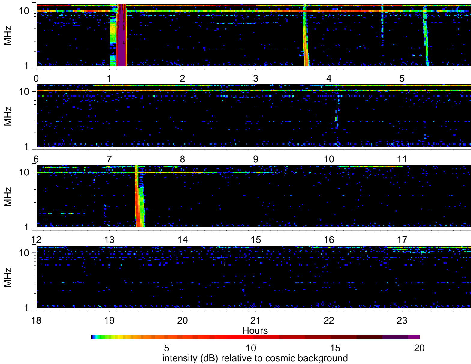
Wind Waves RAD2 receiver: 2005/8/30
