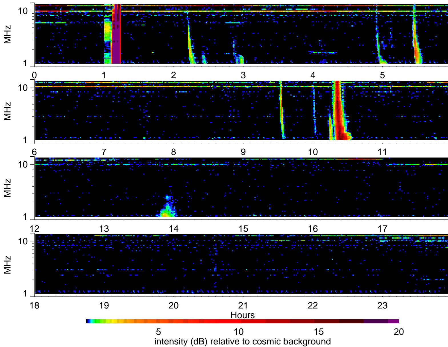
Wind Waves RAD2 receiver: 2005/8/28
