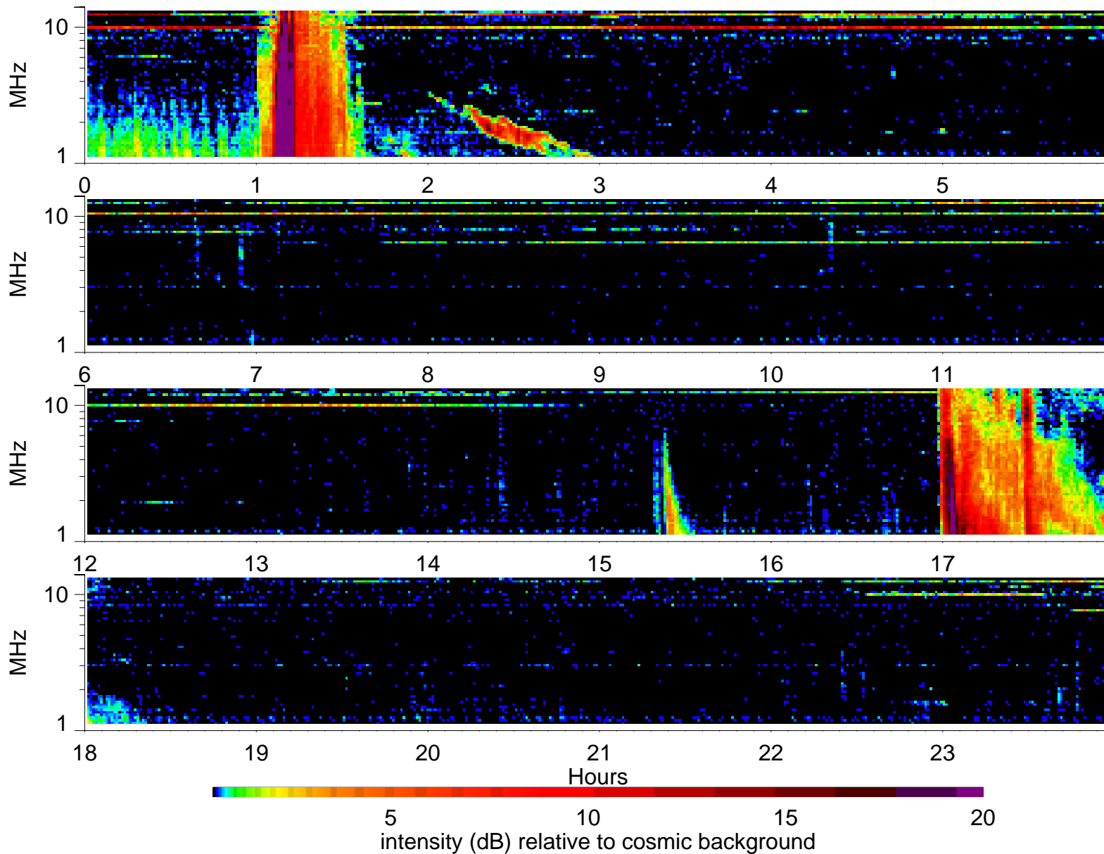
Wind Waves RAD2 receiver: 2005/8/22
