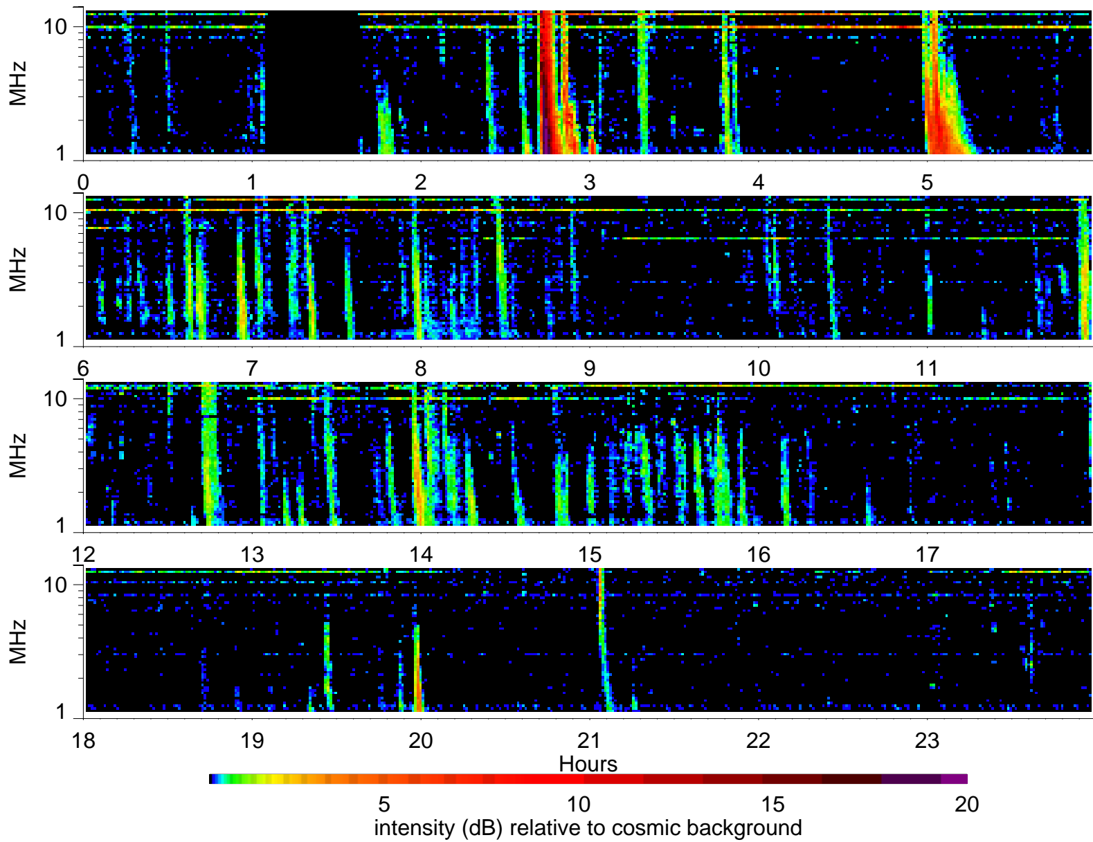
Wind Waves RAD2 receiver: 2005/8/3
