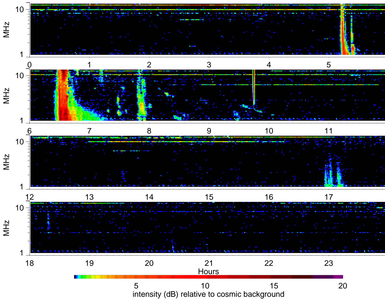
Wind Waves RAD2 receiver: 2005/7/30
