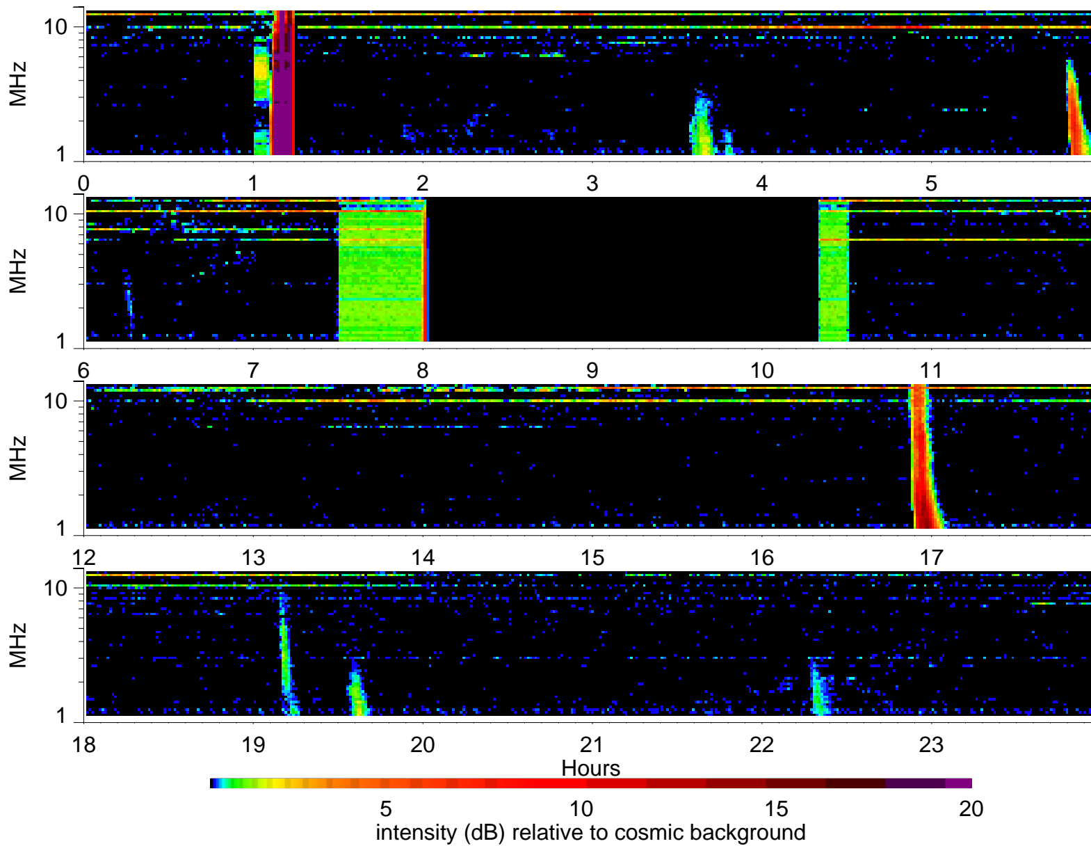
Wind Waves RAD2 receiver: 2005/7/21
