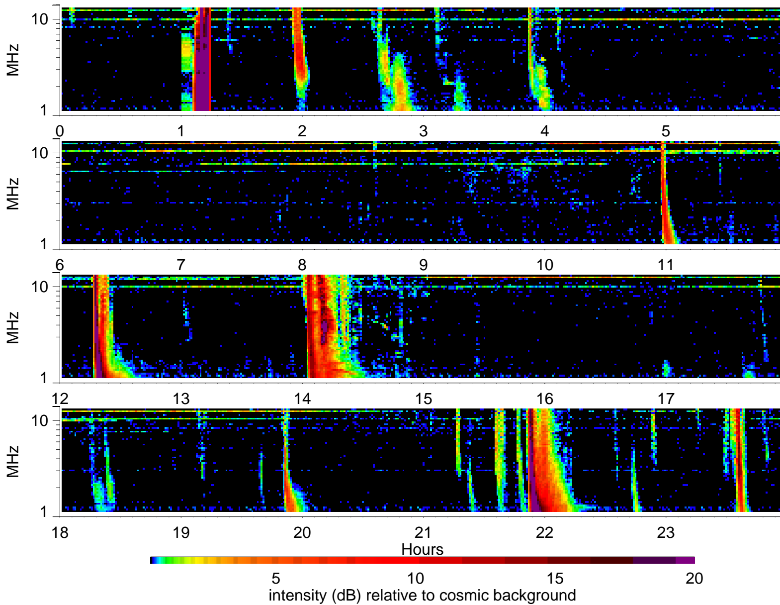
Wind Waves RAD2 receiver: 2005/7/13
