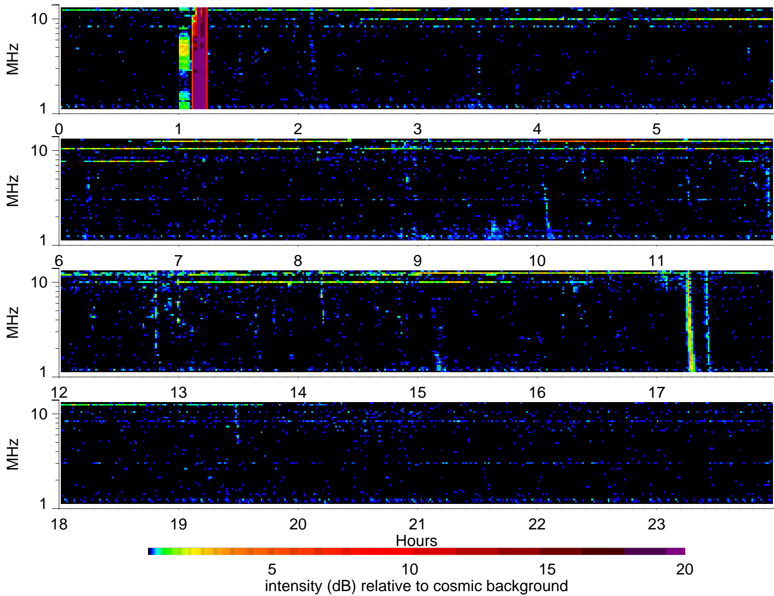
Wind Waves RAD2 receiver: 2005/7/5
